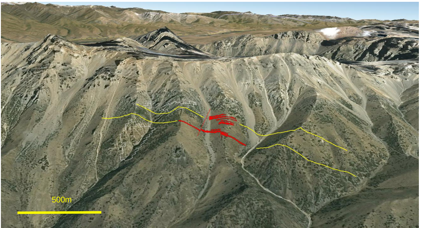
Figure 1 The surface outcropping Aucu high grade gold resource (red outlines) with exploration in 2015 planned to test the extensions shown in yellow.
