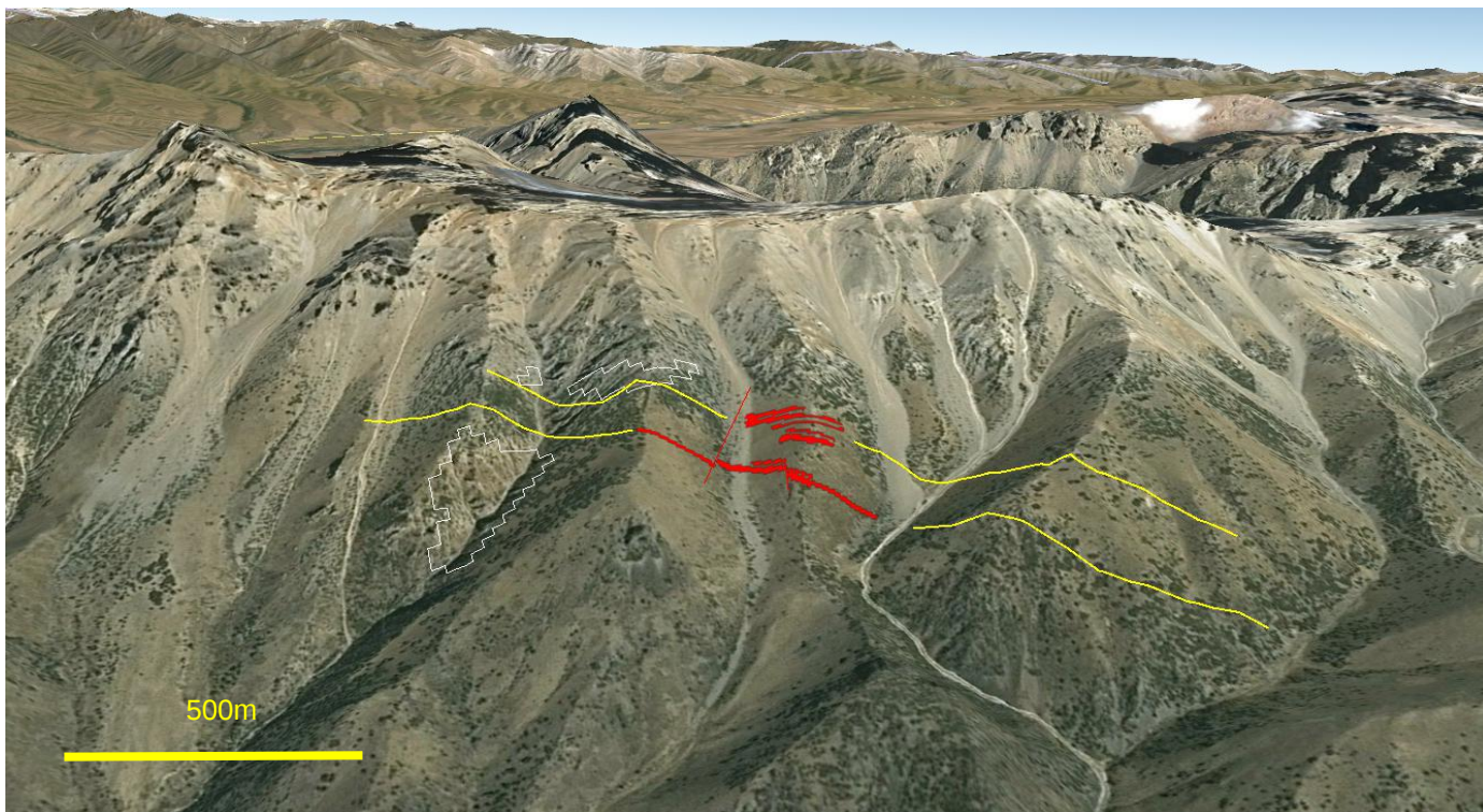
Figure 3 The surface outcropping Aucu high grade gold resource (red outlines) with exploration in 2015 planned to test the extensions shown in yellow.
