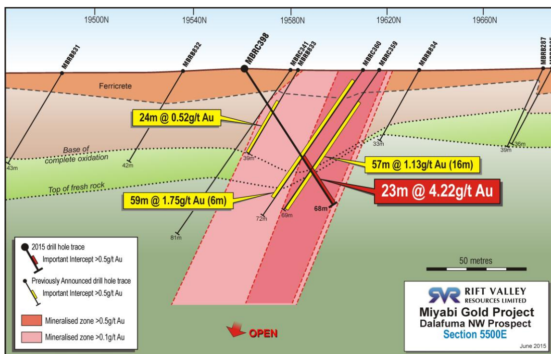
Figure 5: Dalafuma Northwest Cross Section 5500E
