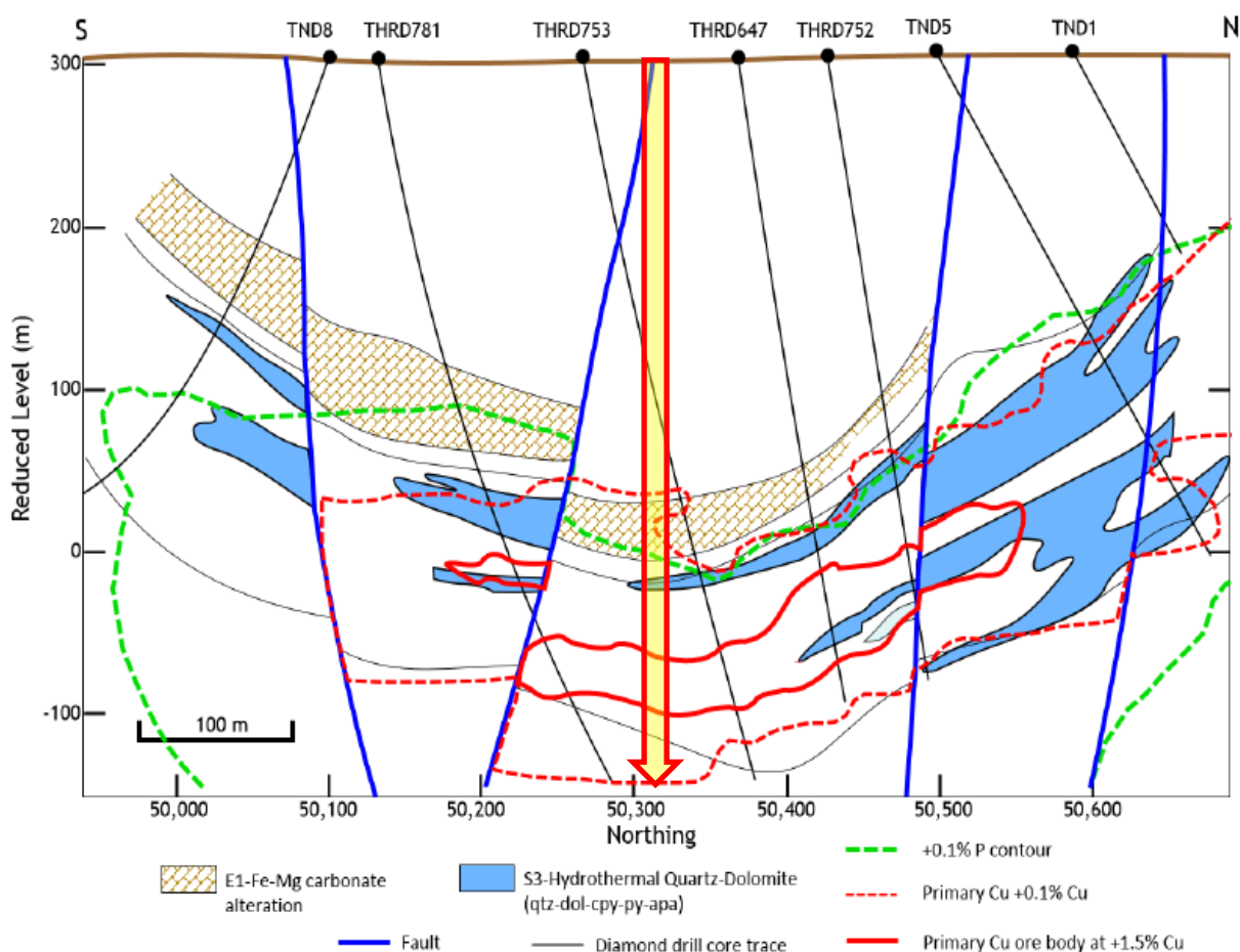
Figure 3 The “Nifty” Model after Anderson, 1999, with the drillhole represented as the arrow above and schematically below in Figure 4
