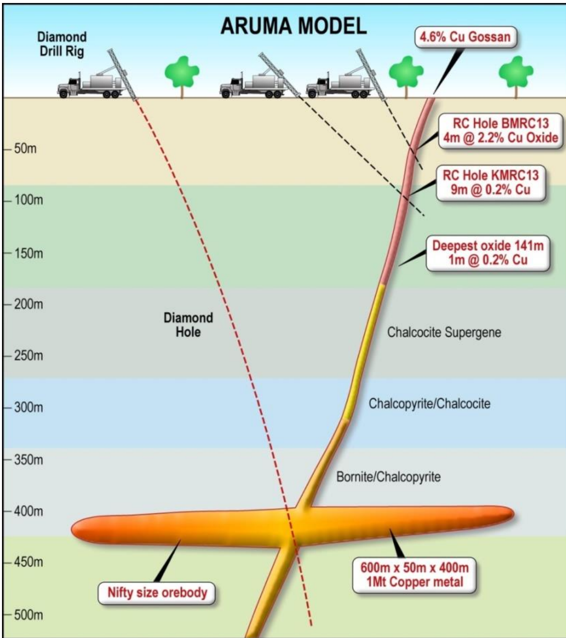
Figure 4 Schematic section and drill hole to test the Nifty Model.
