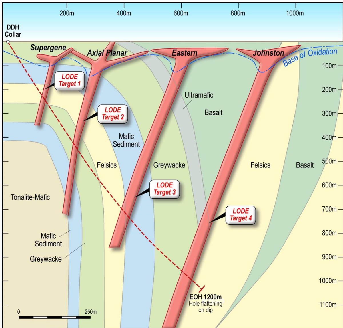
Figure 2 Schematic section of the EIS drill hole (Figure 1) with predicted structure and geology (Looking North West)
