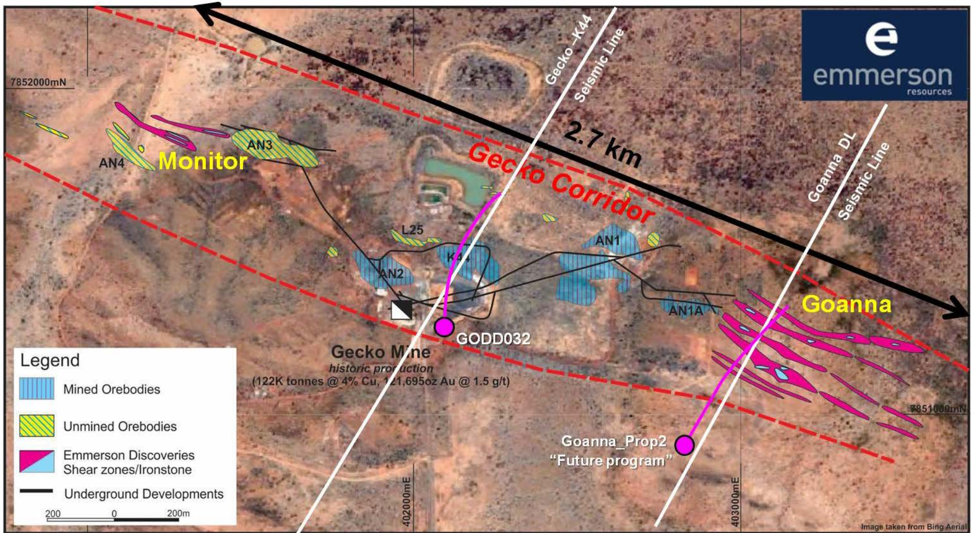
Figure 1: Plan view of the Gecko Corridor, showing the location of GODD032, the position of the 2D seismic lines and location of the Goanna prospect.
