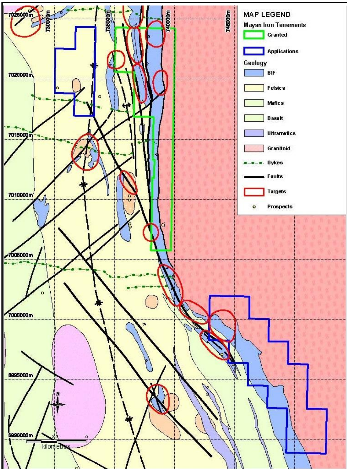
Figure 2 – Geological interpretation of the Gidgee region.
