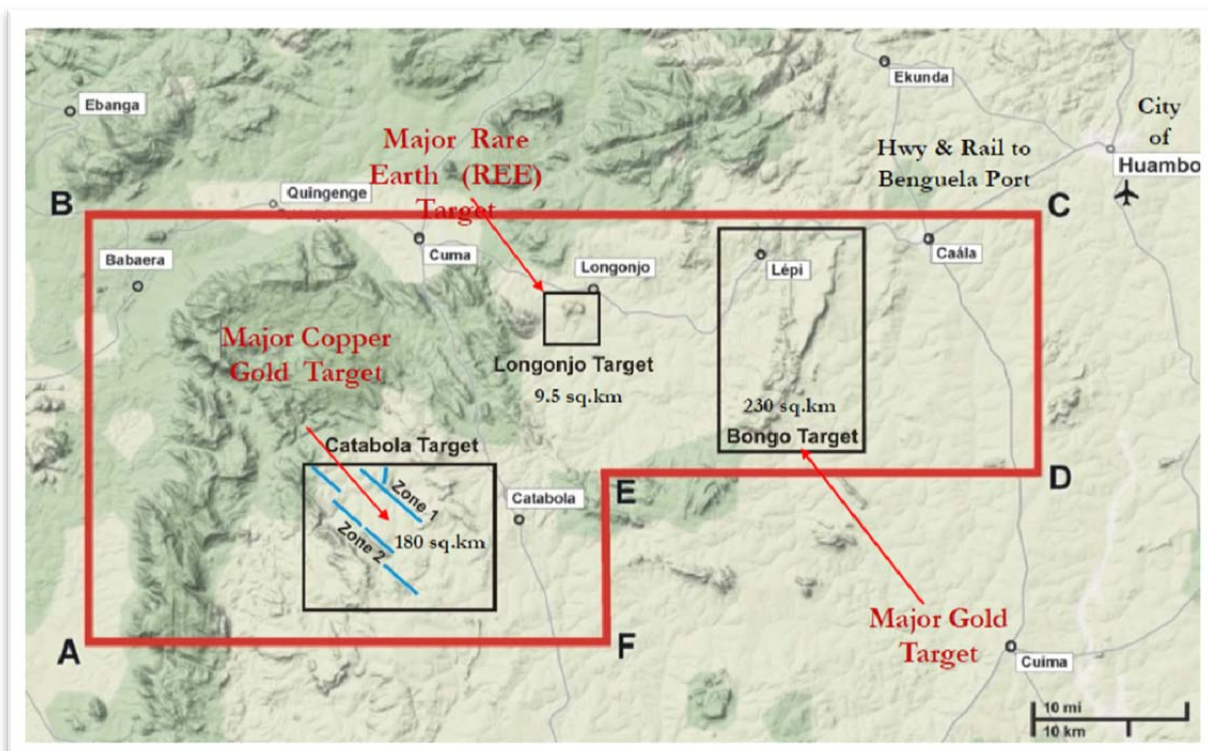
Figure 4: Ozango project showing Longonjo REE Prospect and other major targets
