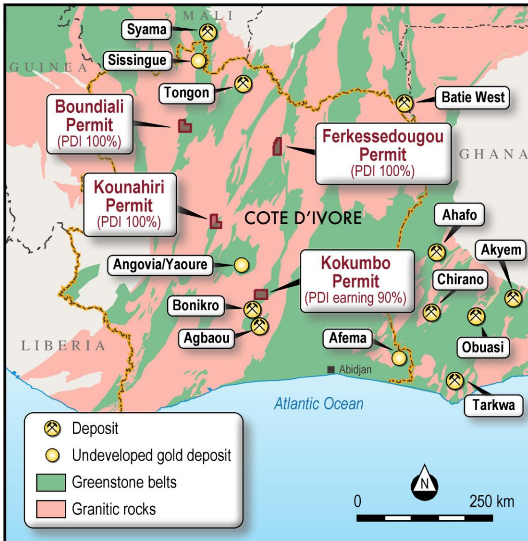
Figure 2: Locality map of PDI permits in Cote D'Ivoire
