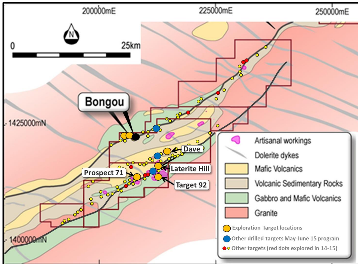
Figure 1: Locality map of PDI permits near Bongou in eastern Burkina Faso, showing Bongou gold deposit and prospects which make up the Exploration Target 1 .
