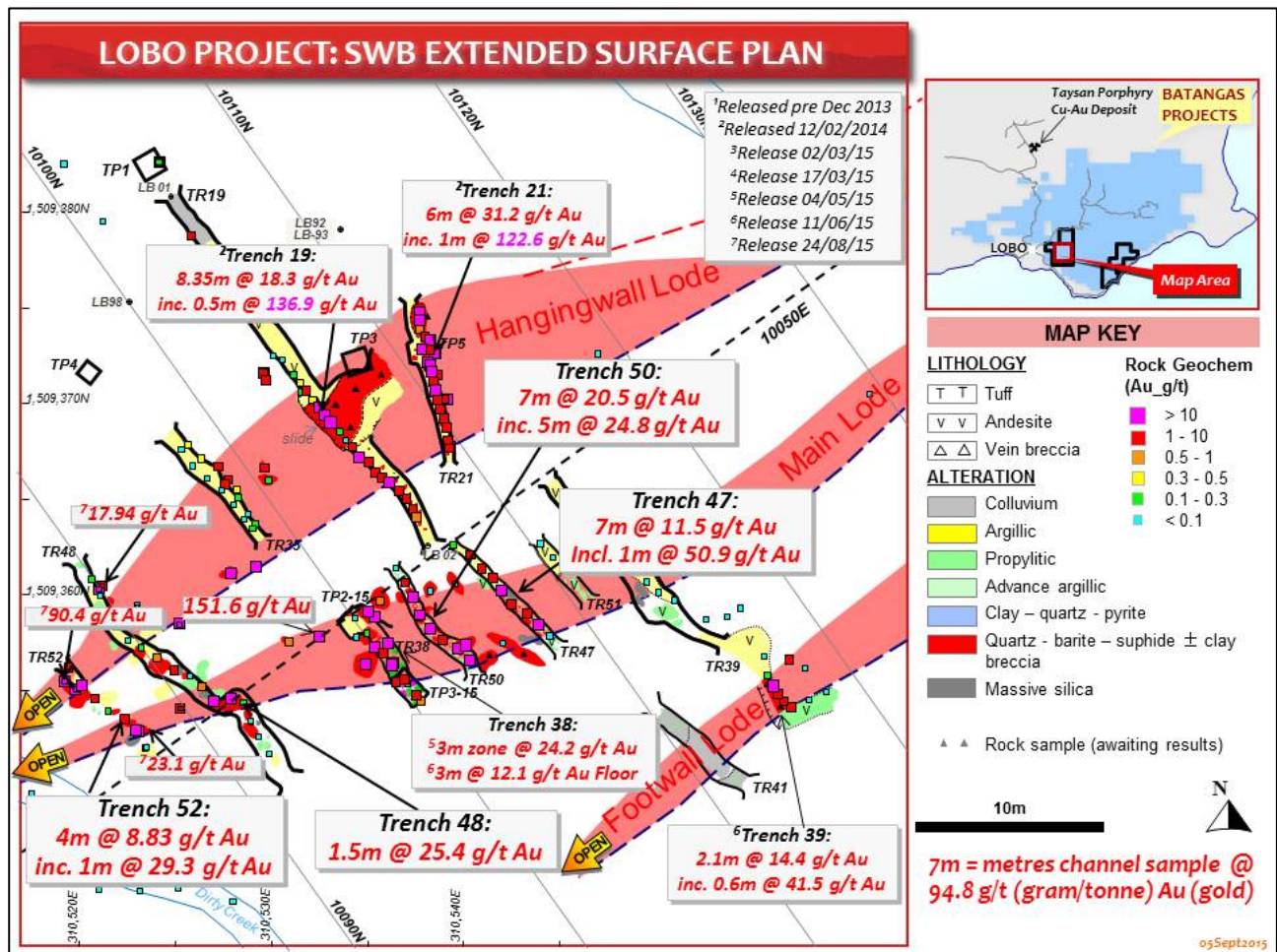
Figure 1: Plan of South West Breccia Extended, Lobo Prospect, with new high grade surface results
