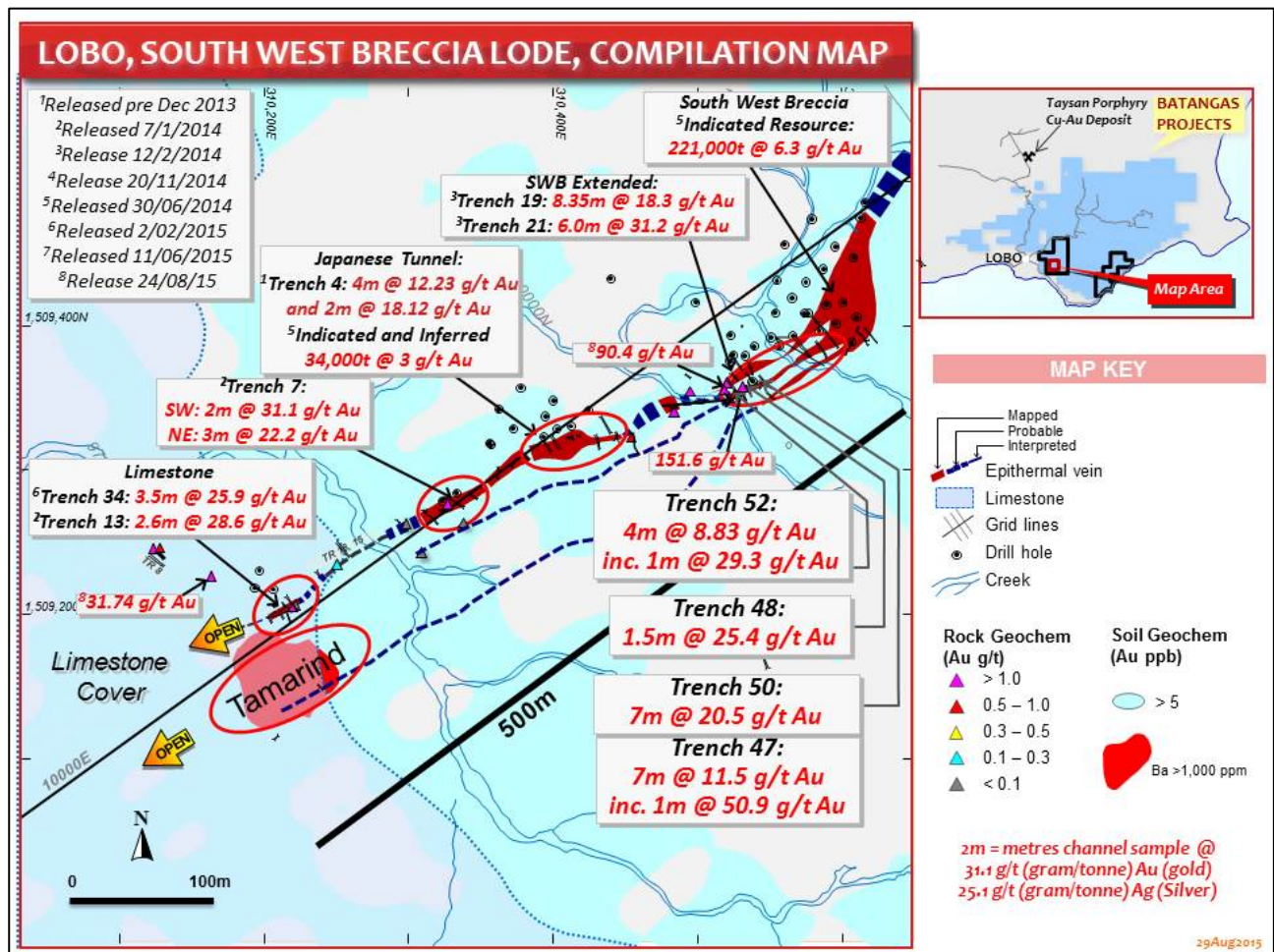
Figure 2: Plan of South West Breccia Lode structure with new high-grade results
