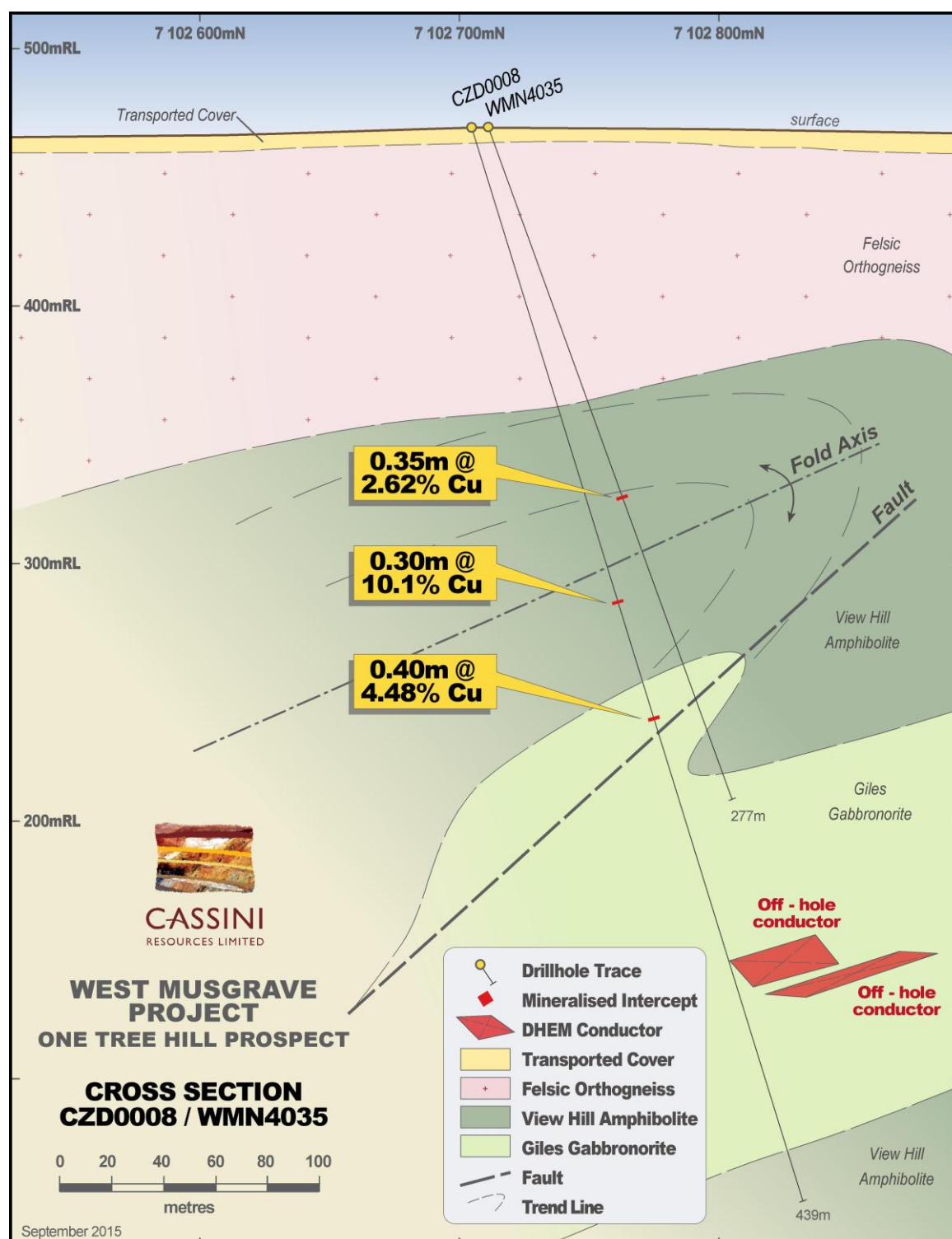
Figure 1. Cross section of CZD0008 with WMN4035 showing DHEM conductors and drill results
