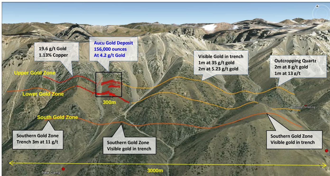
Figure 7 Aucu Gold deposit (black box) and locations of visible gold identified in outcrop and trenches. Yellow and orange traces are mineralised zones.
