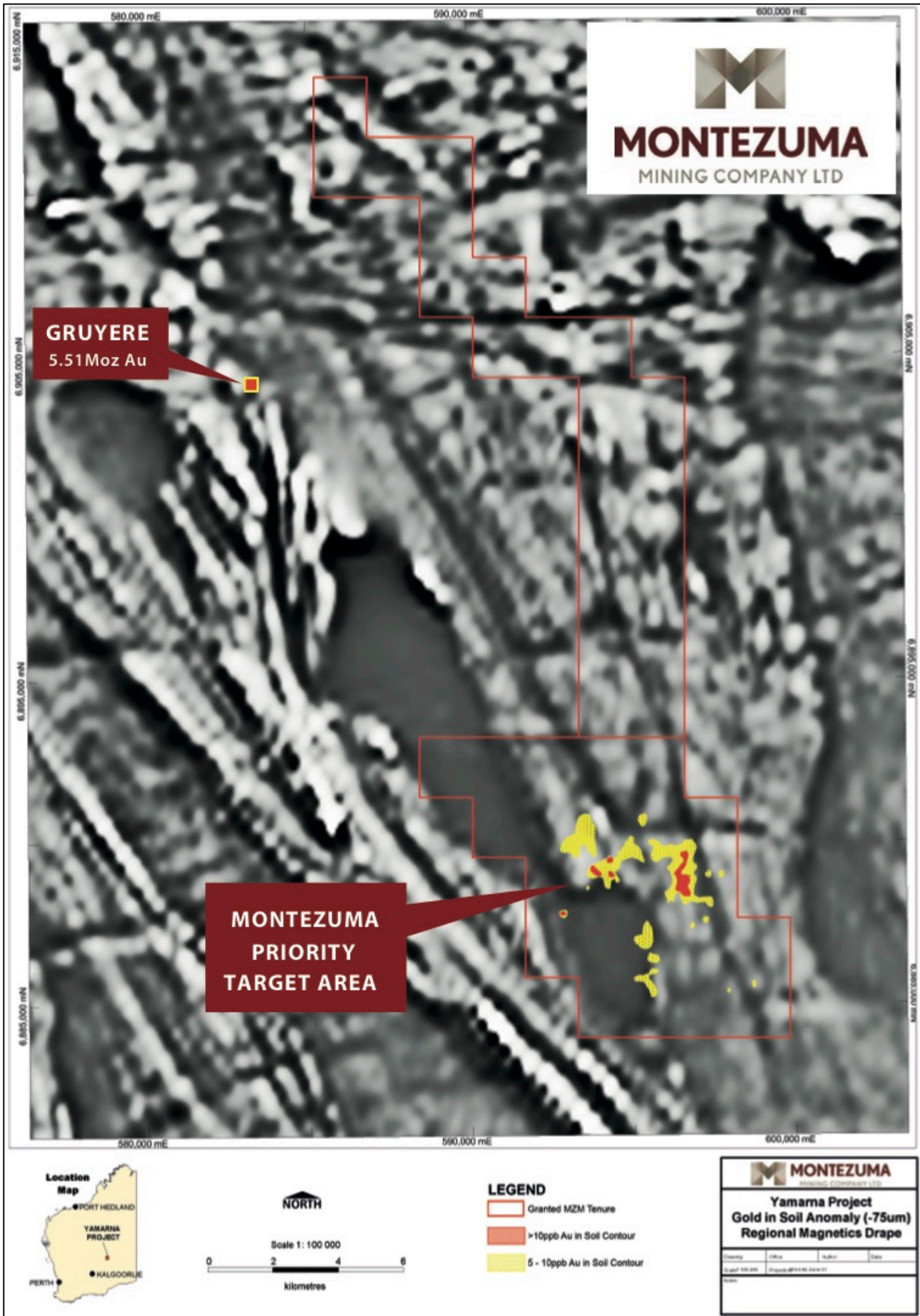
Figure 2: Gold in soil anomalies generated by Montezuma’s recently completed soil sampling programme over regional aeromagnetics.
