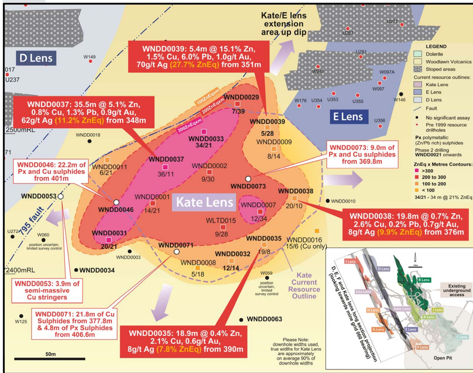
Figure1: Kate Lens Long-Section looking east with recent intercepts shown. Down-hole intercept thickness and ZnEq grade contoured to show relative accumulation of metals across the lens. Current resource outline is shown for reference.
