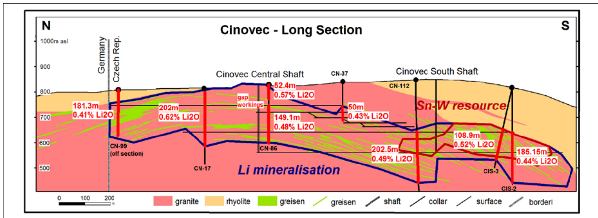
Figure 1 – Cinovec schematic long section showing select lithium drill intercepts
