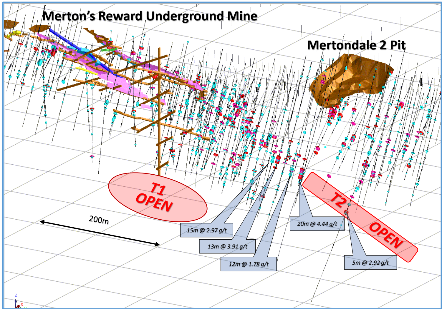
Oblique view of Merton's Reward (looking up along the stoped intershear lodes in pink) highlighting the two targets areas (T1+T2) with existing downhole assay data (0.0-1.0 g/t Au=black, 1.0-3.0 g/t Au=cyan, 3.0-5.0 g/t Au=red and >5.0 g/t Au=magenta).
