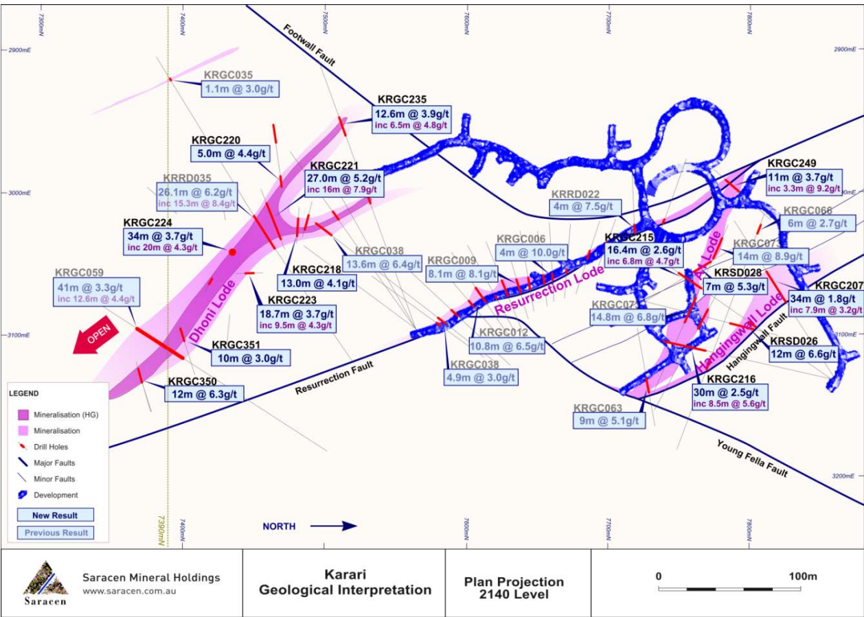
Figure 7 - Karari Plan View
