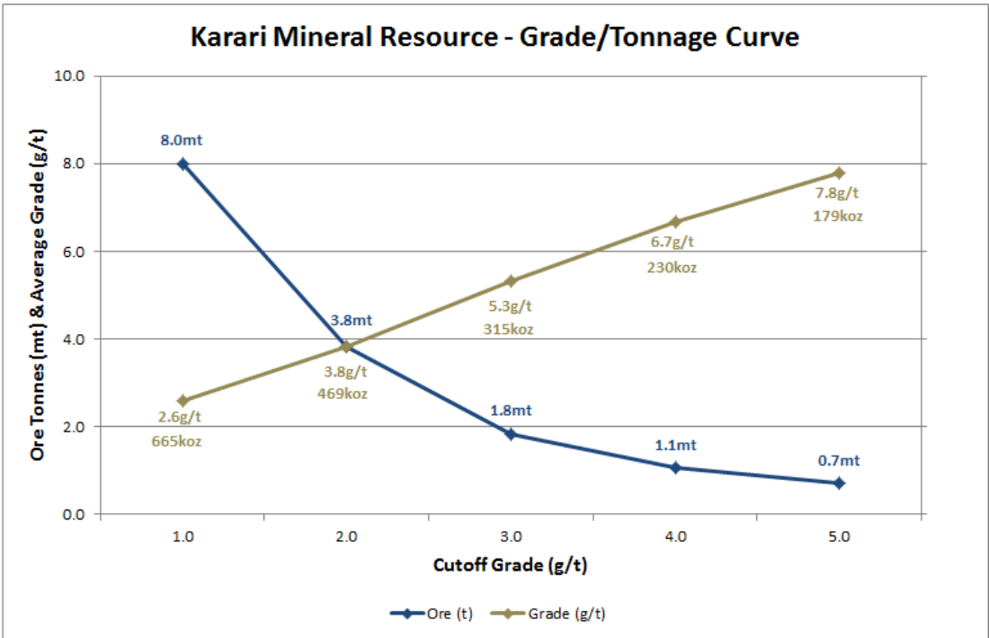
Figure 6 – Karari Grade / Tonnage Curve
