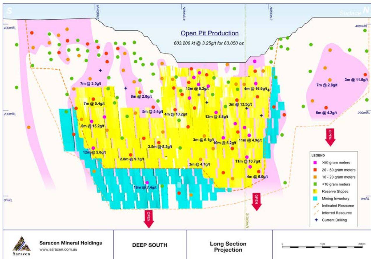
Figure 23 - Deep South Long Section showing Ore Reserve and Mining Inventory
