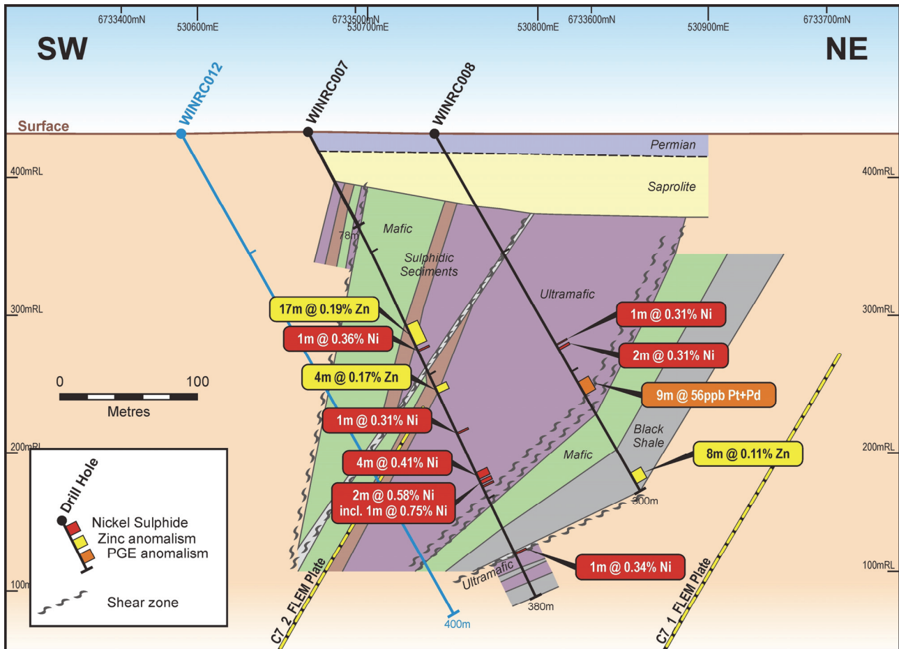
Figure 2 – Interpreted geological cross section of drill holes on the '007 Section' at the Windsor Prospect (+50m), showing nickel sulphide and PGE intersections on the basal ultramafic contact and elevated Zn intersections in adjacent sulphidic sediments. The prospective basal contact will be tested at depth by the planned hole WINRC012 as shown.
