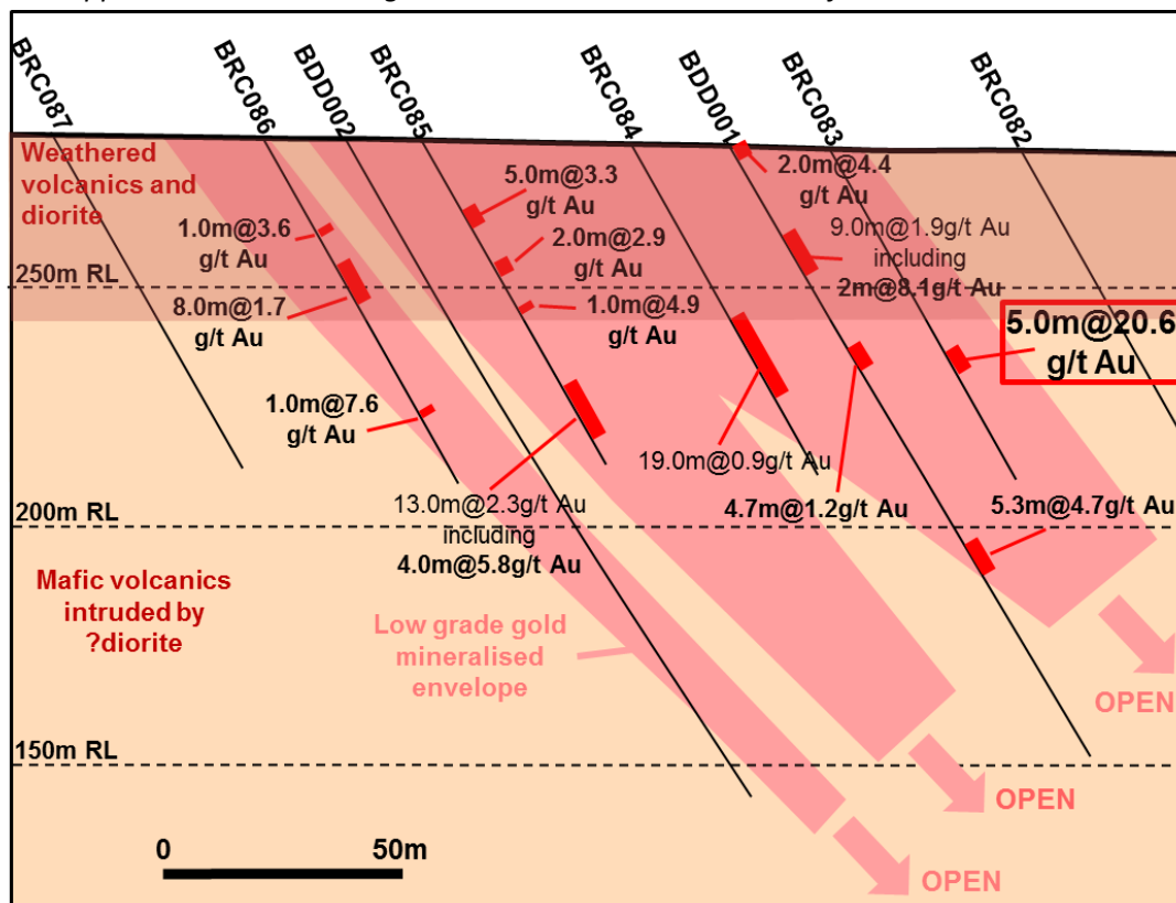
Figure 5: Drill cross section 1 – showing zone with good continuity from hole to hole. Note also apparent enrichment in gold values and widths in near surface weathered zone.
