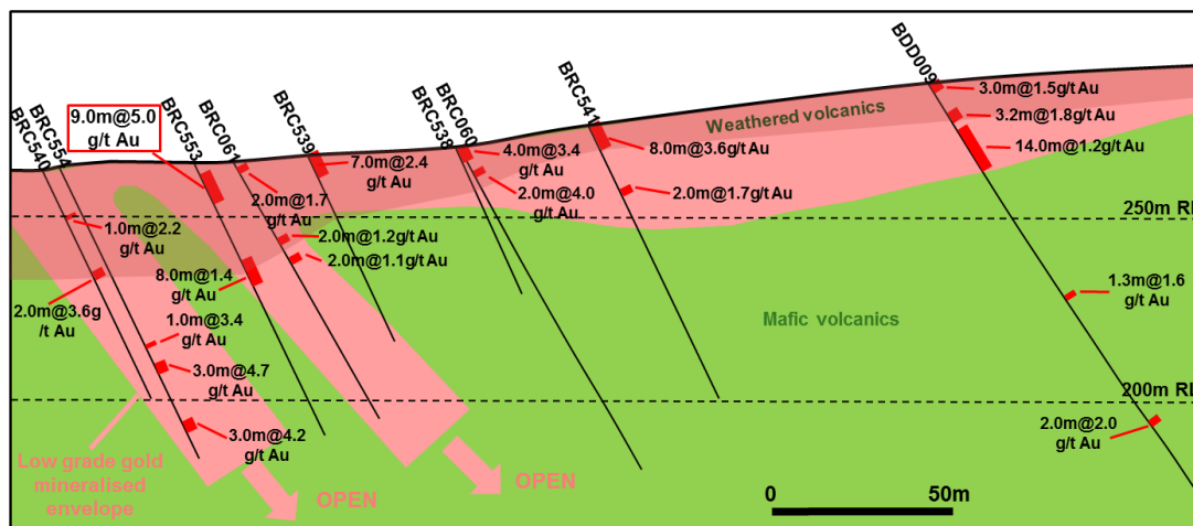
Figure 14: Drill cross section 3 – showing near surface, possibly partly lateritised colluvial/alluvial gold zone. Note high grade, shallow BRC553 intercept.
