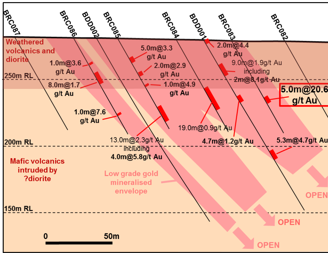
Figure 13: Drill cross section 2 – illustrating uncertain hole to hole continuity with possibility of mineralised zones dipping near parallel to historical drill holes. Note also high grade BRC083 intercept
