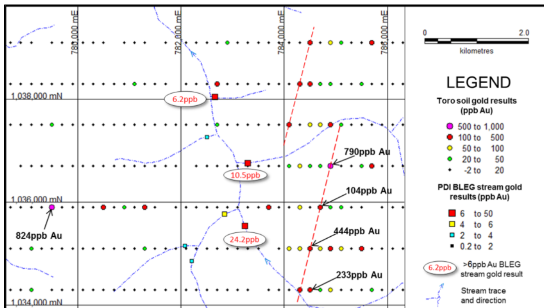
Figure 8: Toro Gold soil sampling grid in the NE portion of the Boundiali exploration permit. Results in grade intervals are shown both for the Toro soil results and PDI's earlier BLEG stream sediment sampling results (reported on 4 th August 2014). Multi-line NNE gold anomalous trends within the broader NE Boundiali anomaly are highlighted.
