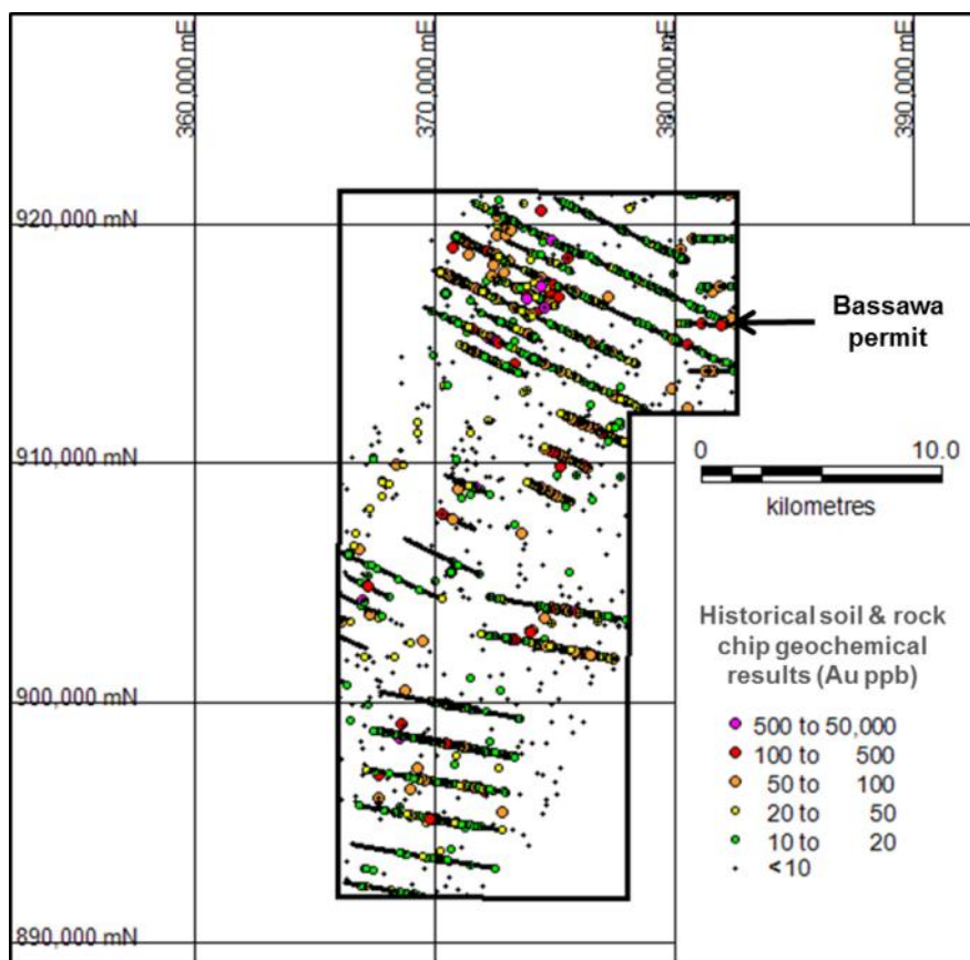
Figure 16: Historical gold in soil and rock chip geochemical values for Bassawa permit.
