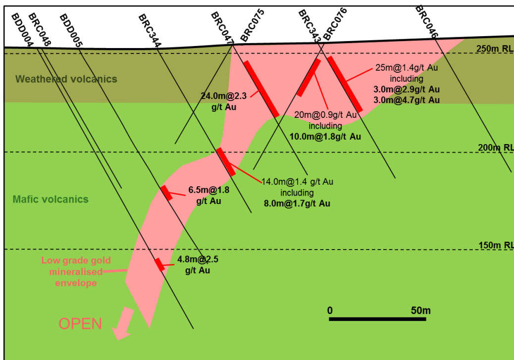
Figure 12: Drill cross section 1 – showing zone with good continuity from hole to hole. Note also apparent enrichment in gold values and widths in near surface weathered zone.
