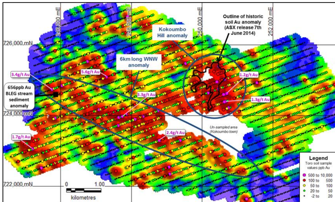
Figure 5: Close-up image of gridded soil, lag and laterite gold geochemical results obtained by Toro, highlighting two major areas of interest – around the old Kokoumbo mine on Kokoumbo Hill and along a 6km long WNW-oriented gold anomaly south and west of Kokoumbo Hill.
