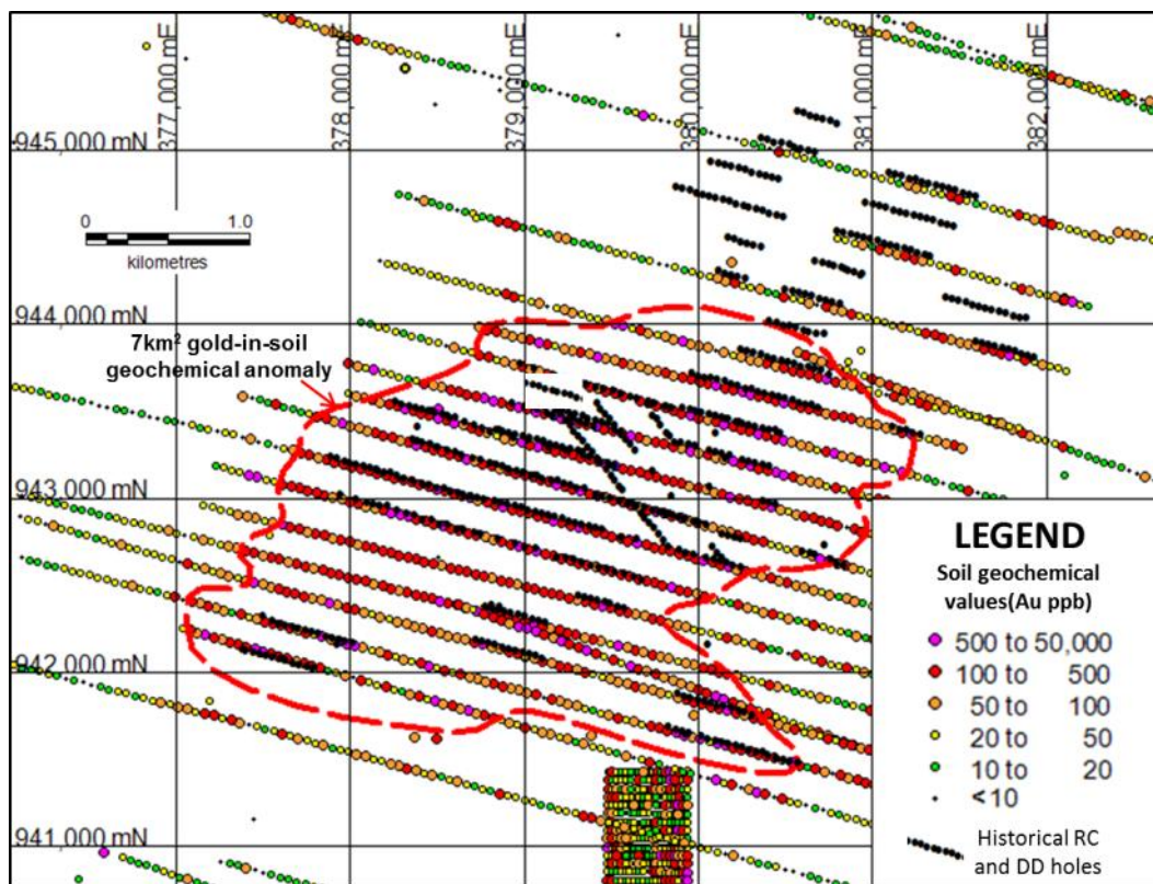
Figure 10: Bobosso gold in soil geochemical anomaly showing values in assay intervals and historical RC and DD holes.
