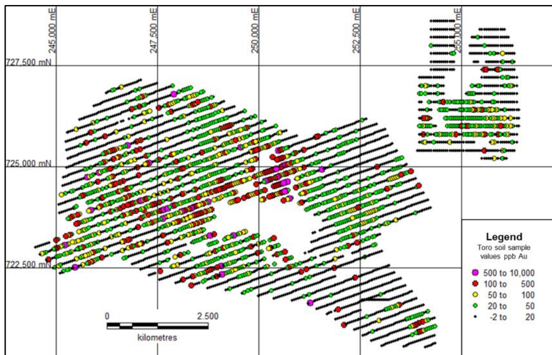
Figure 6: Gold soil geochemistry image showing all Toro Gold soil, lag and laterite sampling results obtained on Predictive's Kokoumbo permit, colour-coded by gold value ranges.
