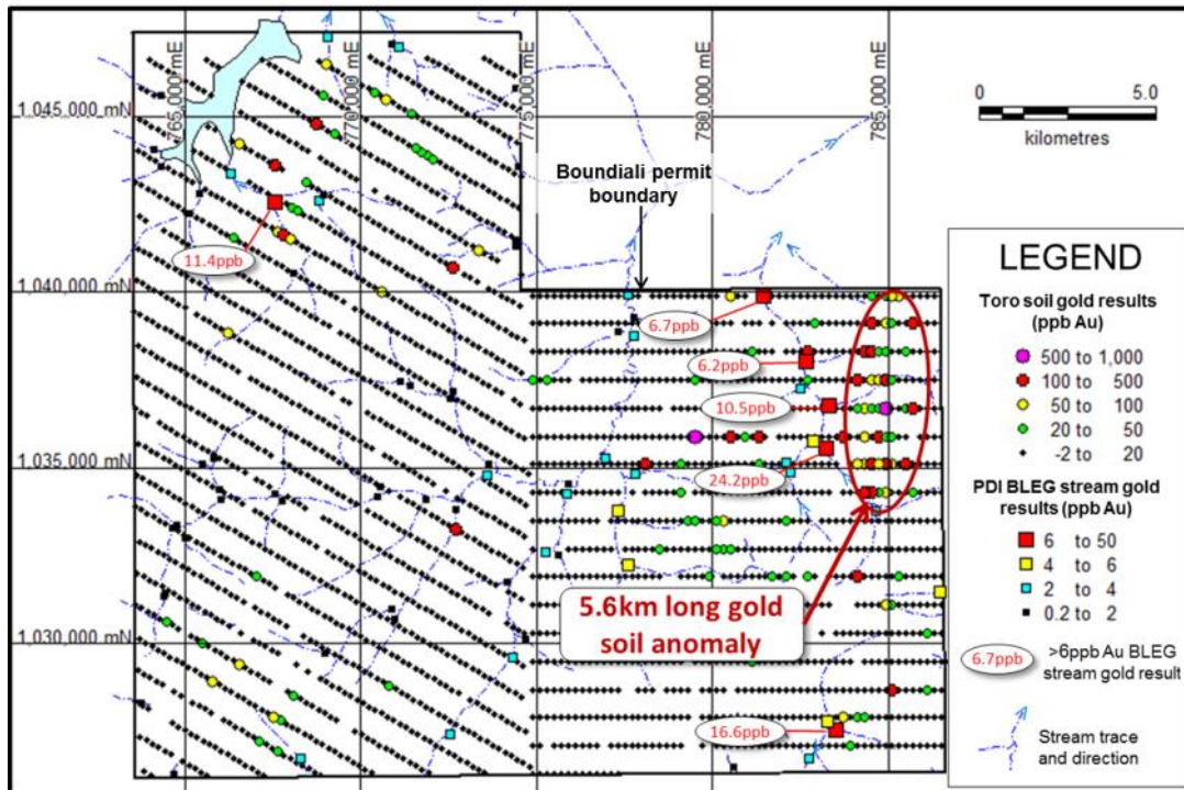
Figure 7: Toro Gold soil sampling grid covering the entire Boundiali exploration permit. Results in grade intervals are shown both for the Toro soil results and PDI's earlier BLEG stream sediment sampling results (reported on 4 th August 2014). The large NE Boundiali gold anomaly is highlighted on this map.
