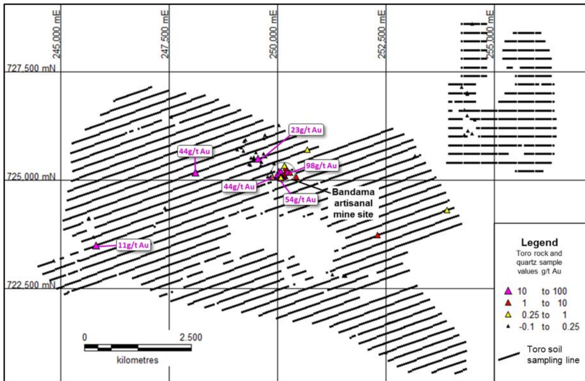
Figure 4: Location of Toro soil sampling grid with location and grade of rock chip and selective quartz samples highlighted
