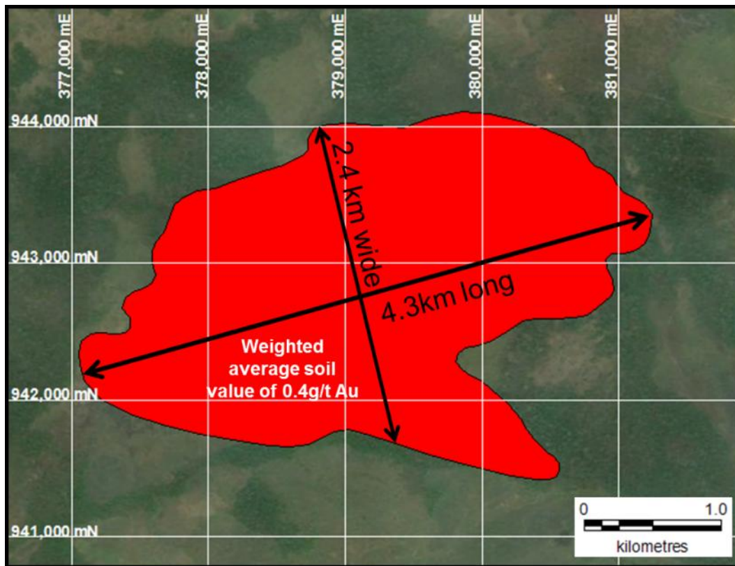
Figure 9: Bobosso gold geochemical anomaly on satellite imagery background
