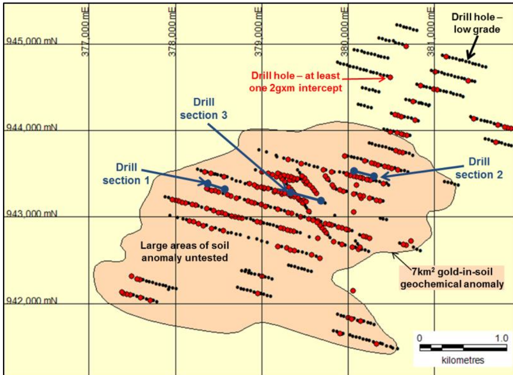
Figure 11: Bobosso gold in soil geochemical anomaly showing location of all historical RC holes, highlighting all holes with gold intercepts of at least 2 g x m and showing cross section locations
