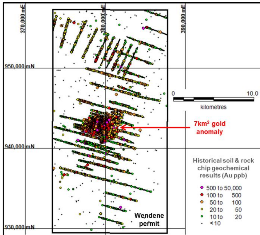
Figure 15: Historical gold in soil and rock chip geochemical values for Wendene permit application.
