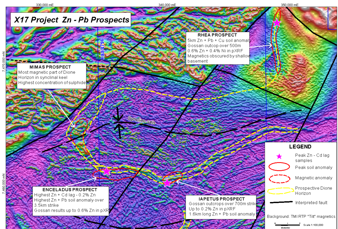
Figure 2. Summary of soil and lag geochemistry and geological interpretation.
