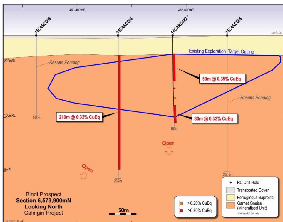
Figure 3 – Bindi Section 6573900mN
