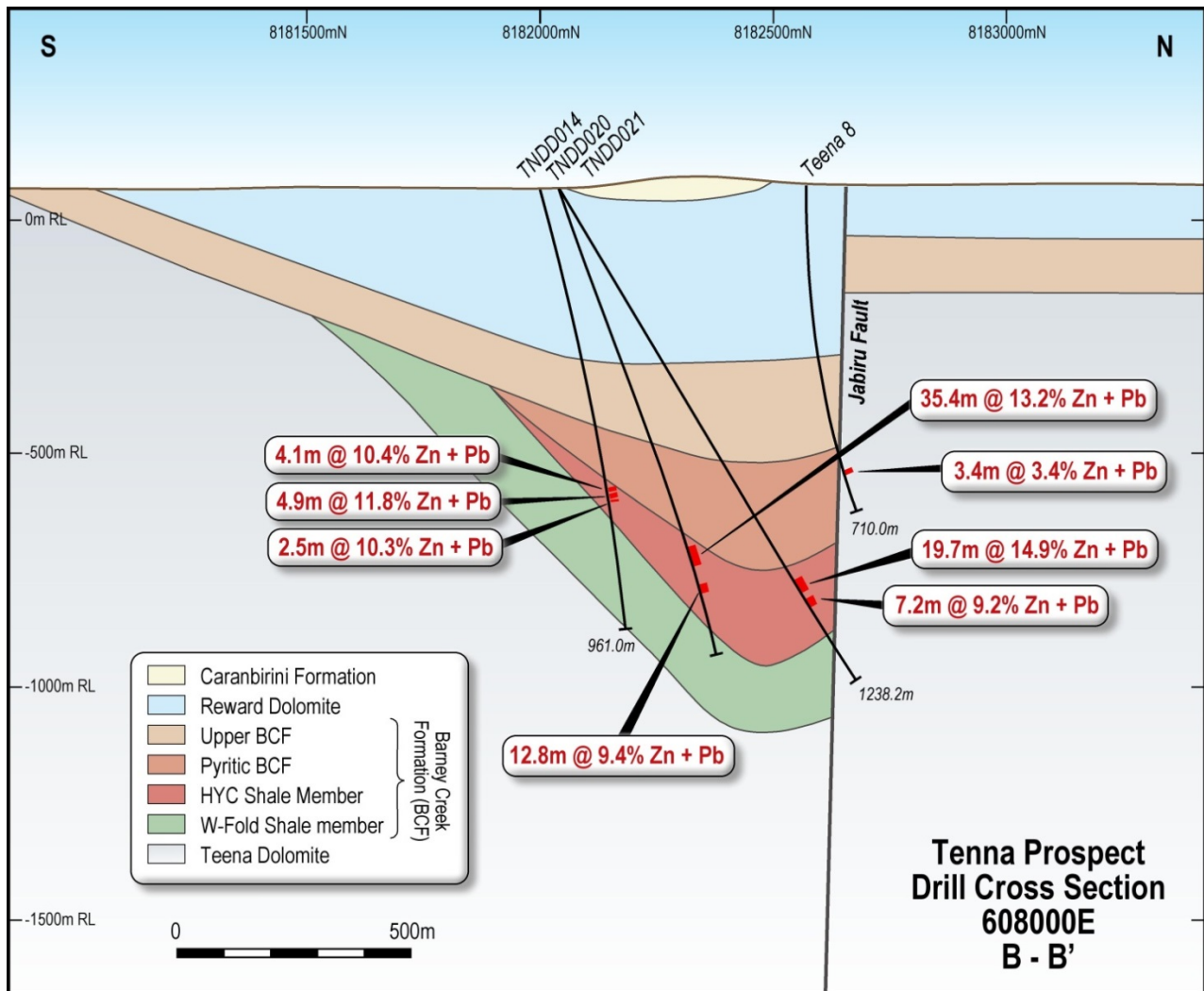
Figure 3: Teena Cross Section B-B', 608000E
