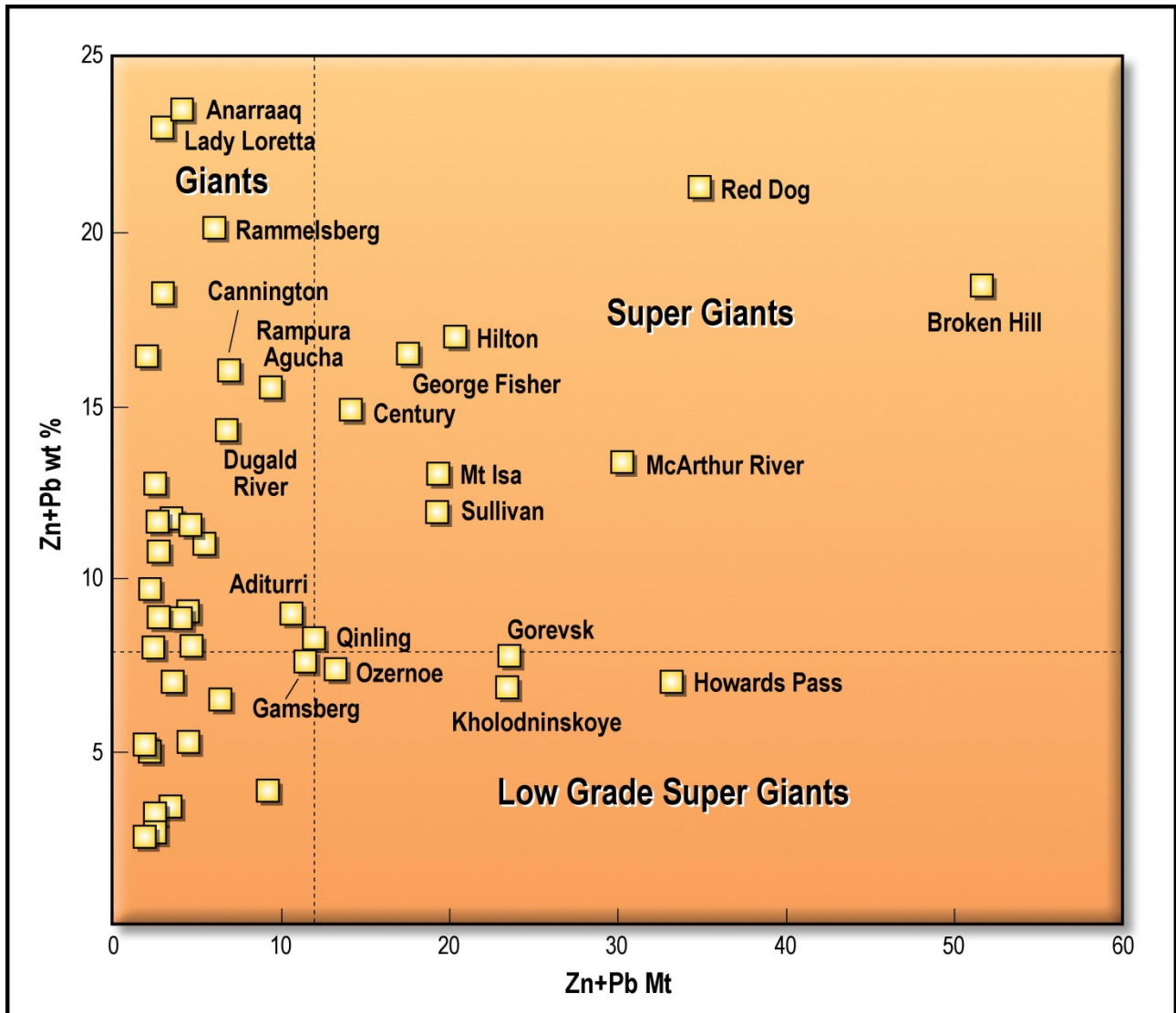
Figure 5: World Sedex Zinc Deposits (after Leach et. al. 2005)
