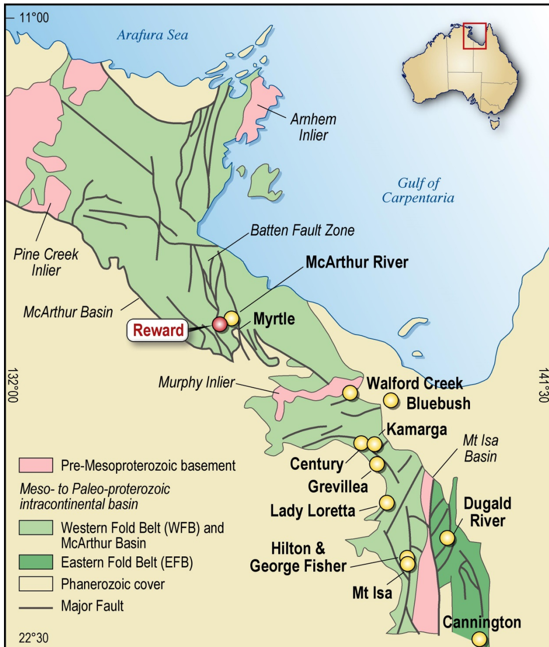
Figure 4: Carpentaria Zinc Province showing the locations of the five major Tier 1 “supergiant” zinc-lead deposits - Mt Isa, Hilton, George Fisher, Century and McArthur River; and the three Tier 2 “giant” deposits, Cannington, Dugald River and Lady Loretta. Other deposits shown are smaller in size.
