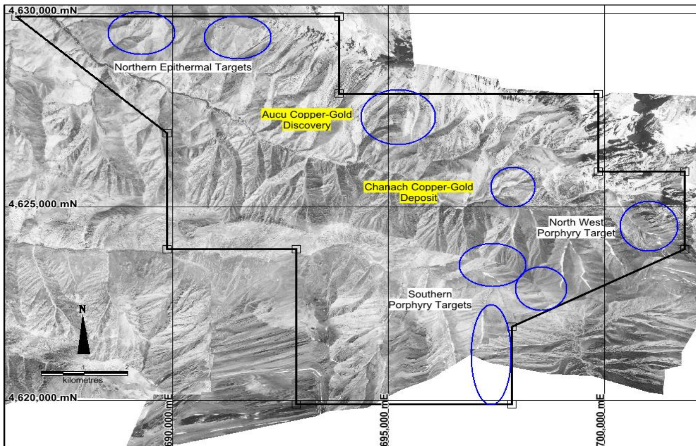
Figure 2 Map showing Chanach license outline and location of the Aucu gold discovery 2.5 km to the NNW of the original Chanach copper deposit.
