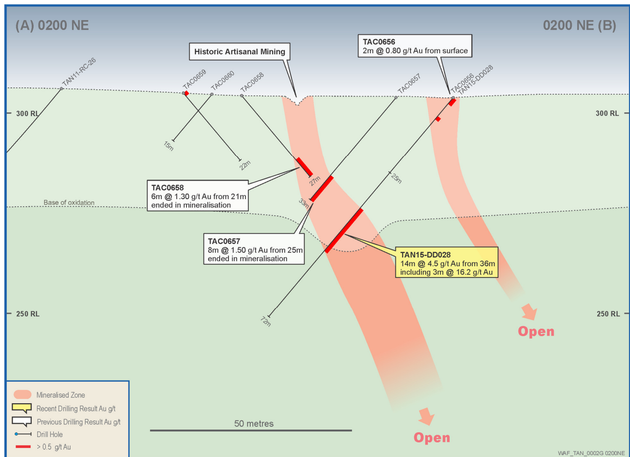
Figure 1: Mankarga 1 Cross-section
