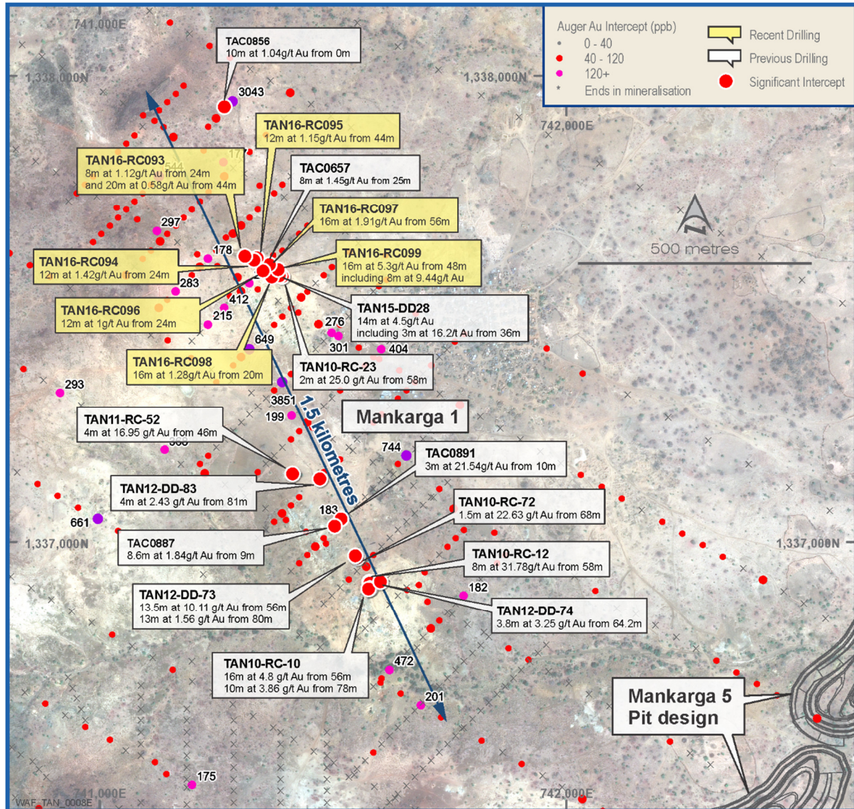
Figure 2: M1 Summary Plan
