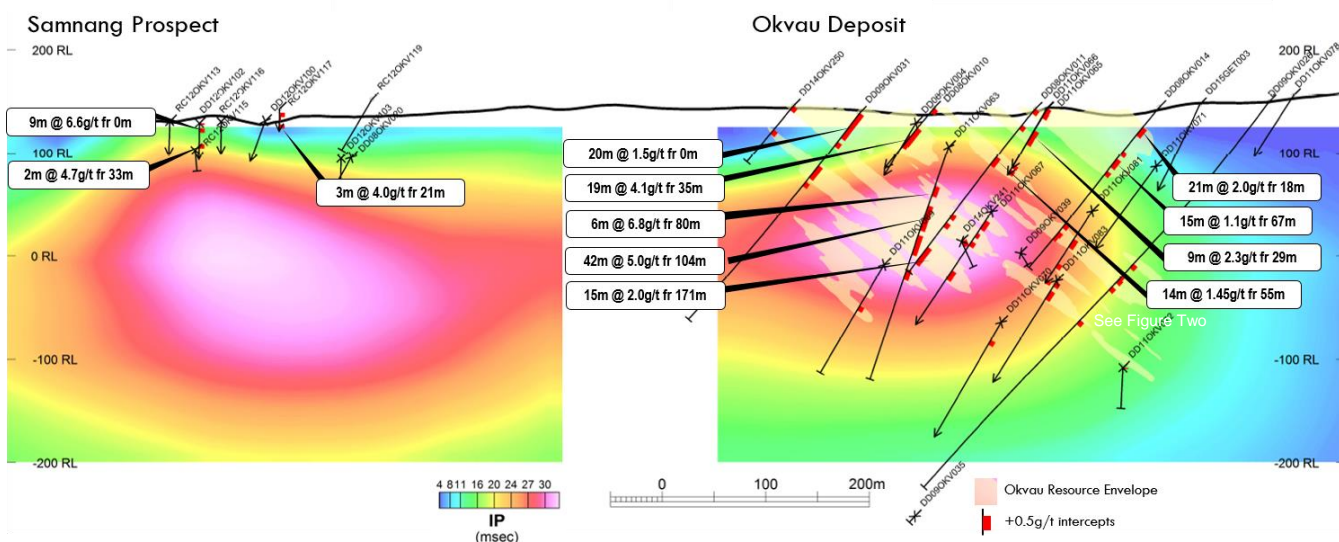
Figure Four | IP Chargeability Cross Section
