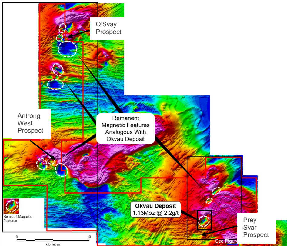
Figure Five | Okvau and O'Chhung License Area - Remanent Magnetic Features Analogous to Okvau Deposit
