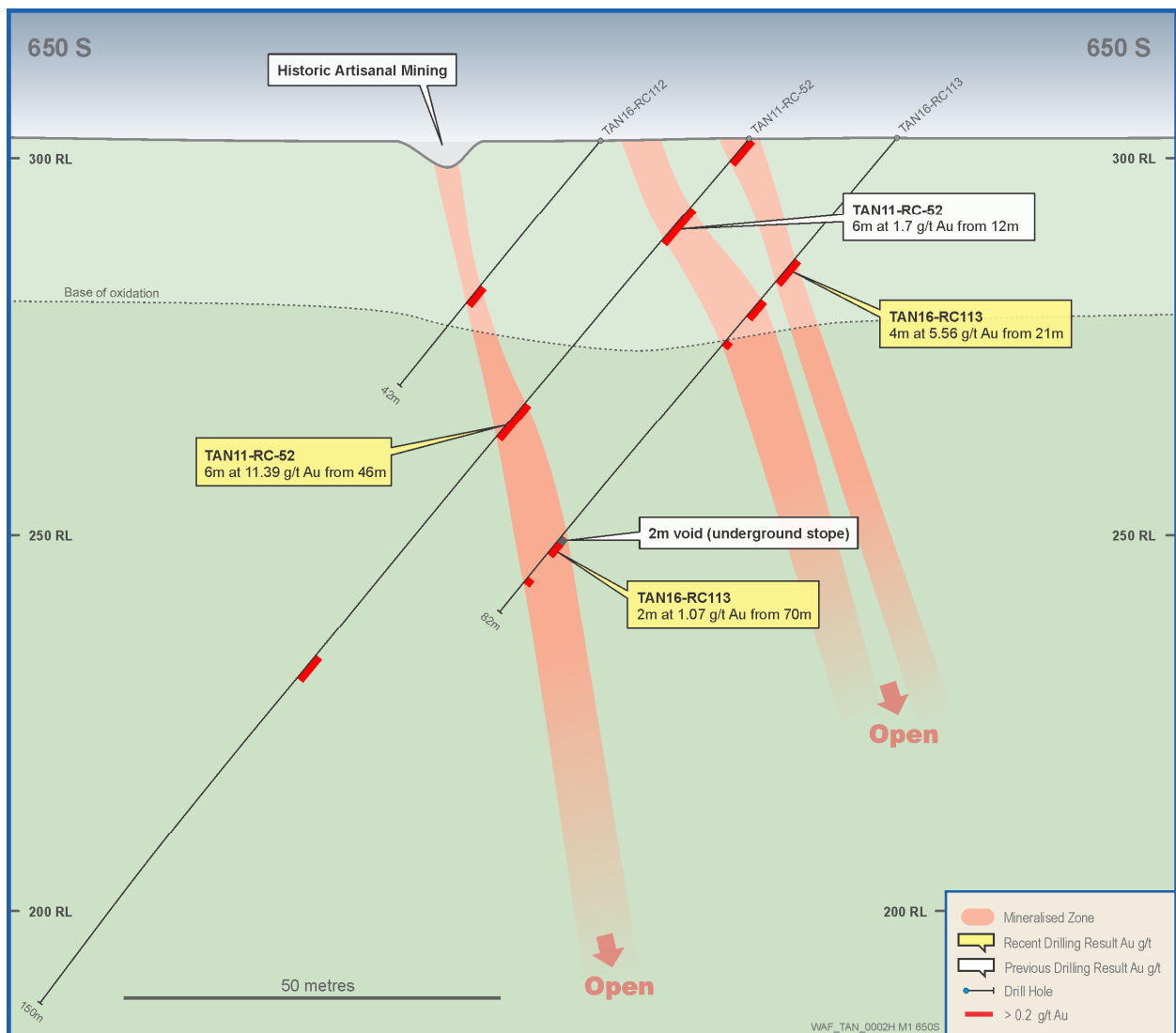
Figure 2: M1 Cross section – SE0650
