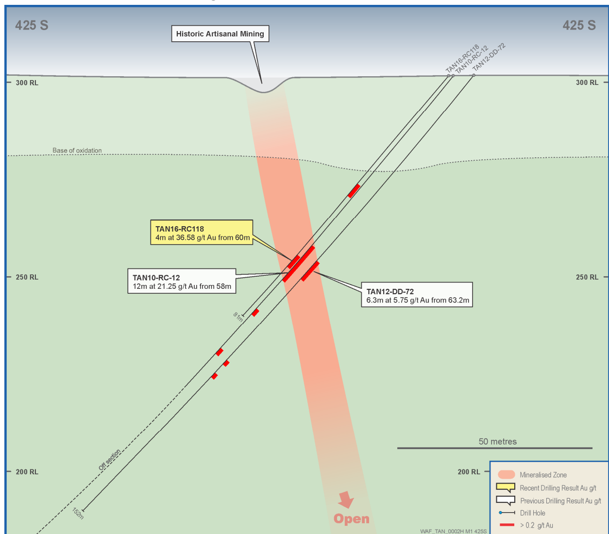
Figure 1: M1 Cross section – SE0425
