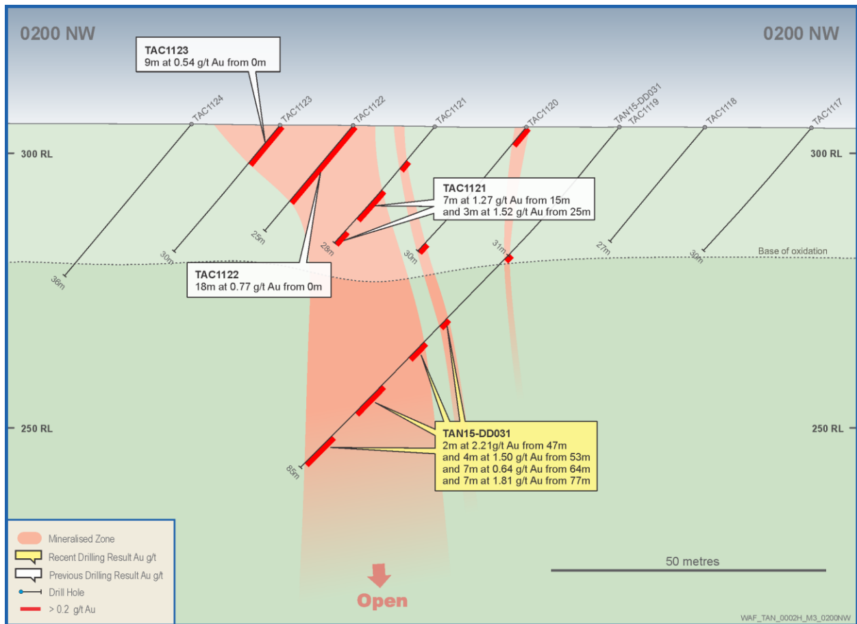
Figure 3: M3 Section
