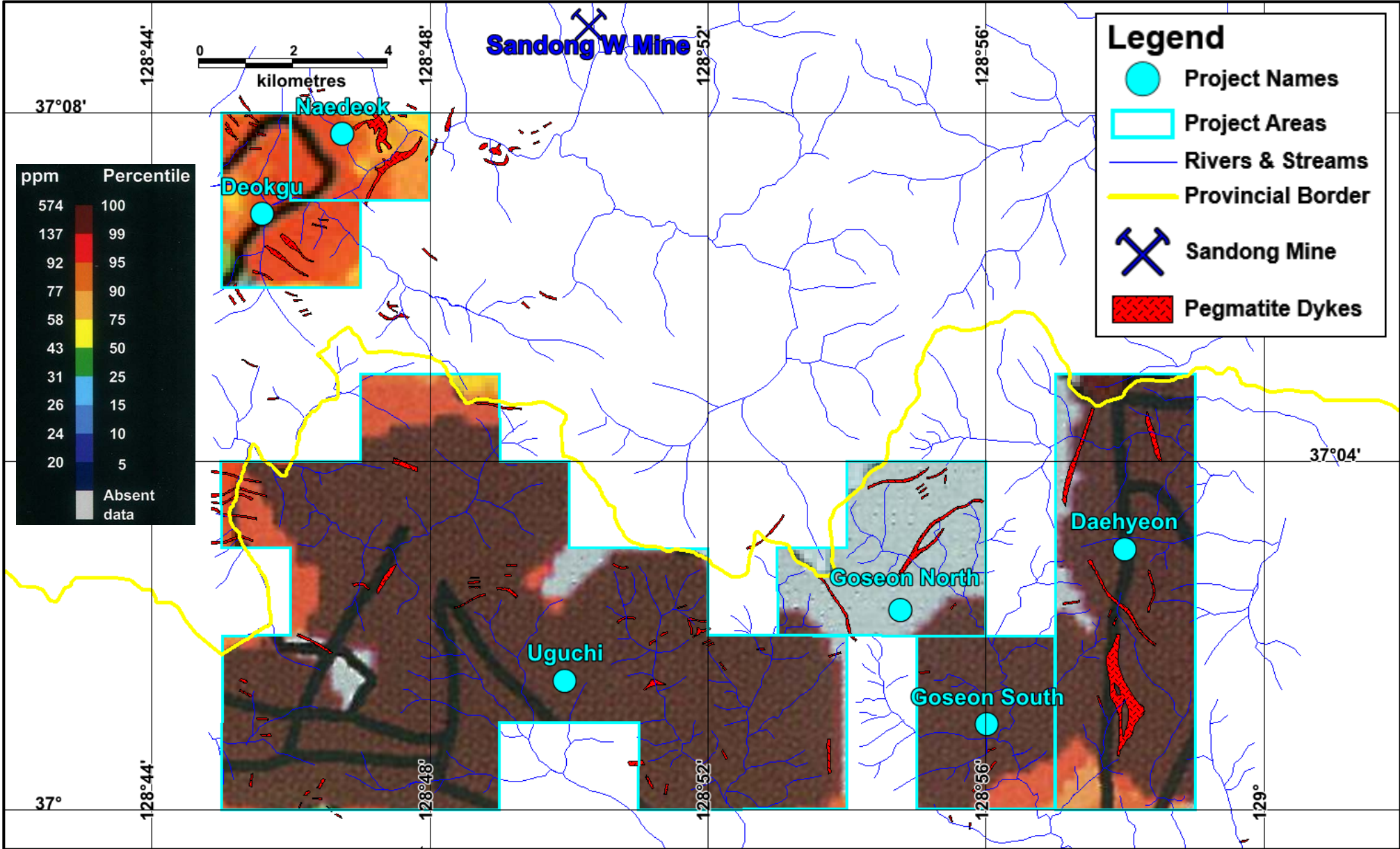
Figure 5: Prospect Areas on the KIGAM stream sediment inverse distance weighted lithium plot 11 . The deeper red-brown colours reflect areas of higher intensity lithium anomalism.
