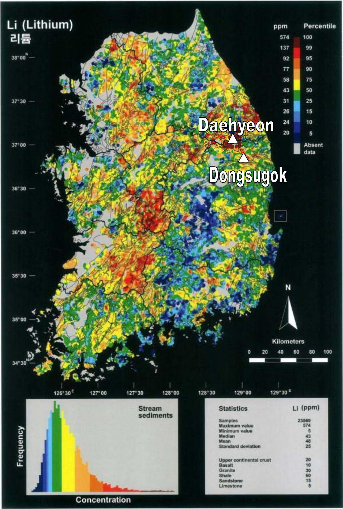
Figure 4: KIGAM Country wide stream sediment data for lithium 11 .
