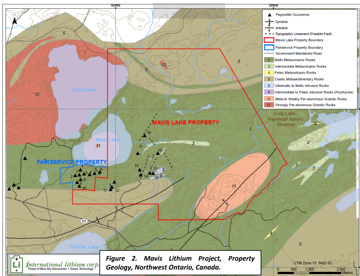
Figure 2a. Project tenure outline, overlaying geology and pegmatite outcrops (numbered)
