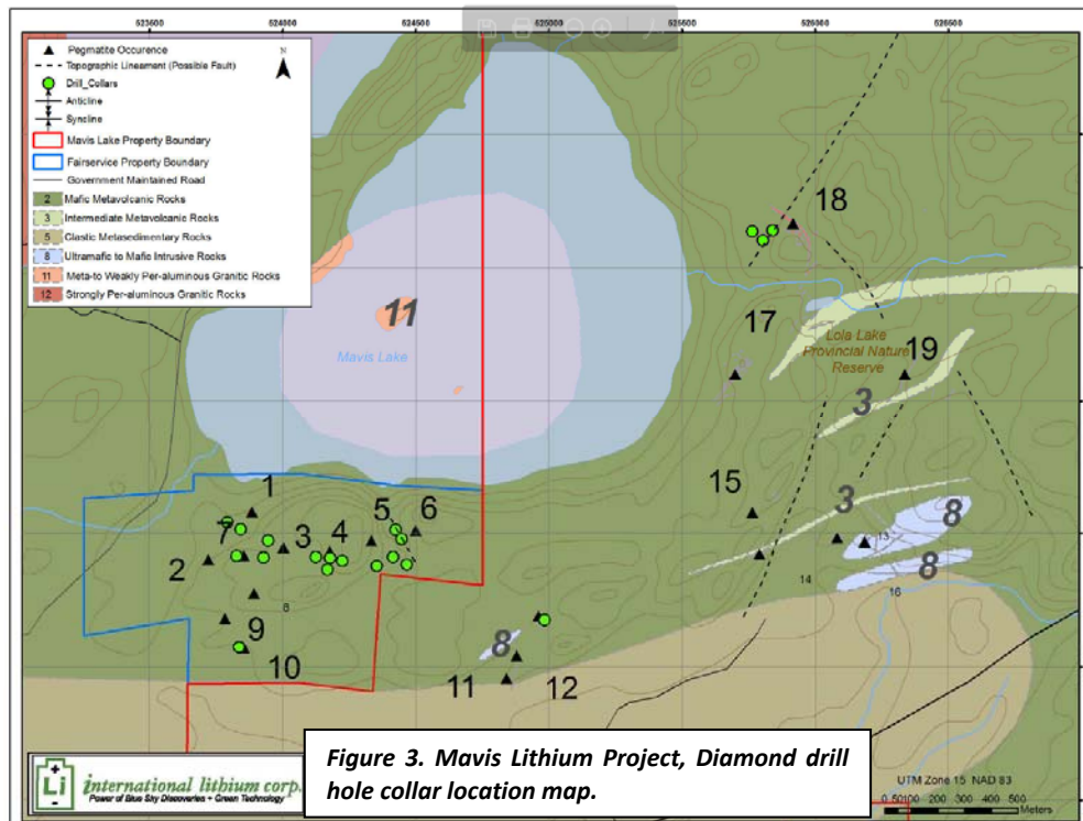
Figure 3. Project tenure outline, overlaying geology and pegmatite outcrops (numbered), showing drill hole collar locations
