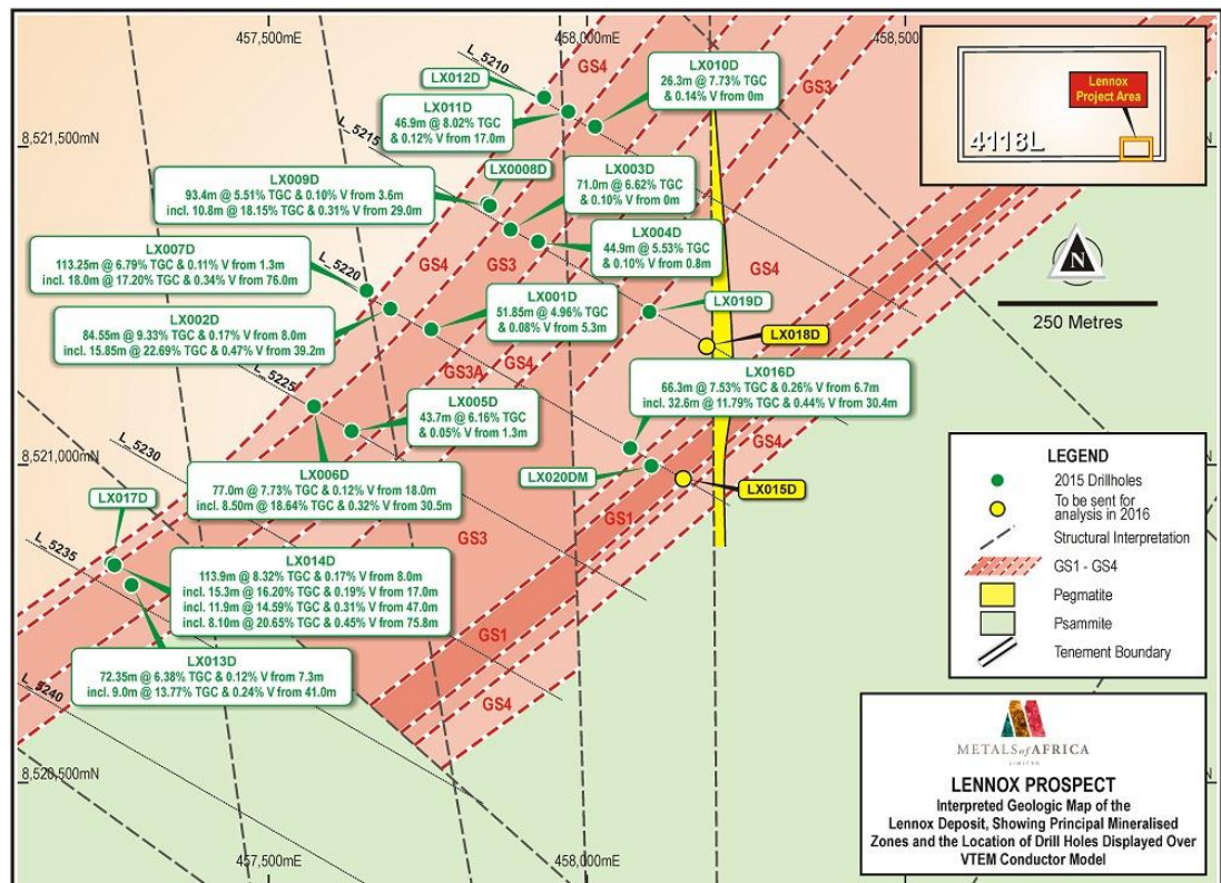
Figure 3 – Interpreted Geological Map of the Lennox Deposit
