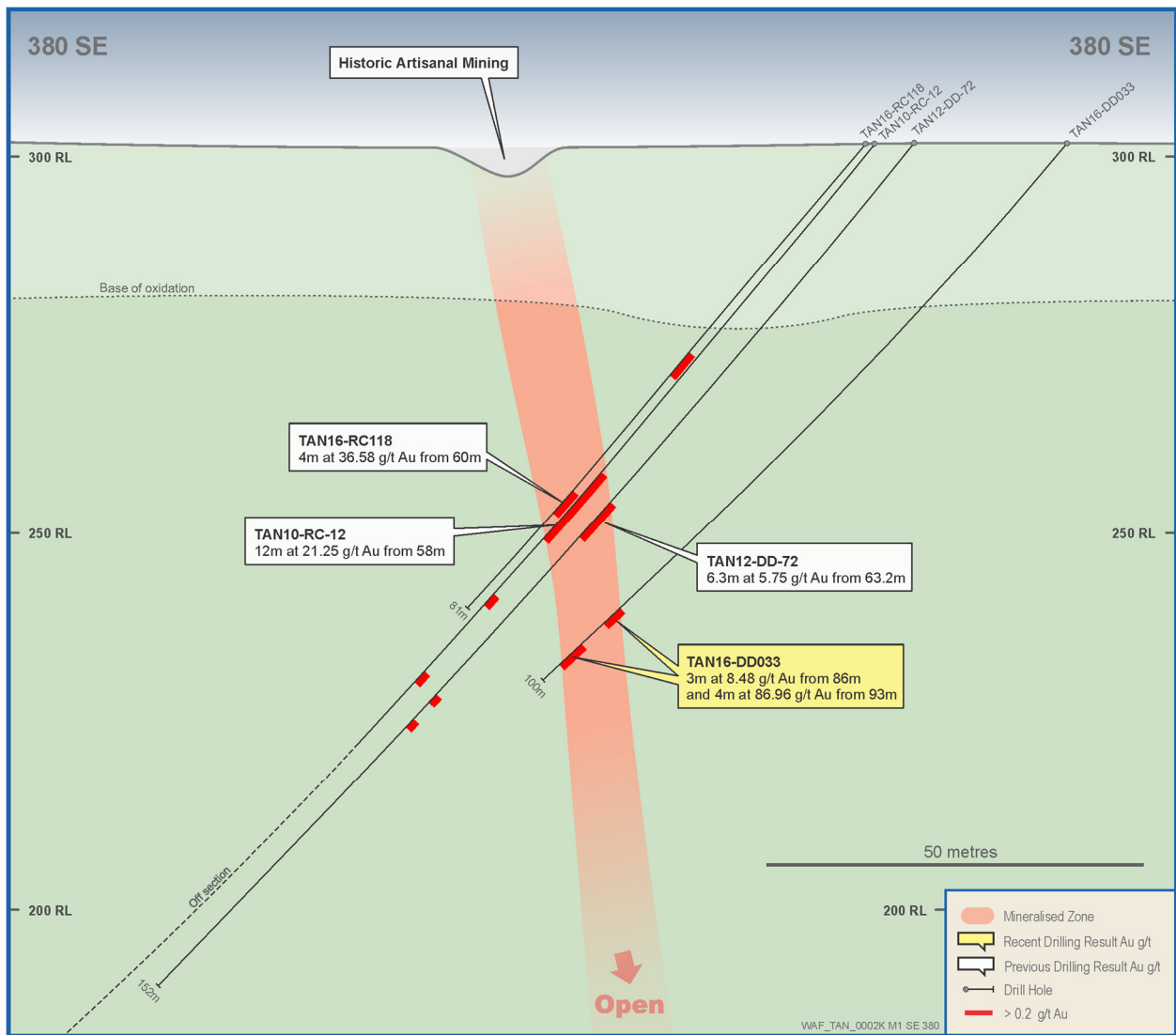
Figure 2: M1 Cross section – SE0380
