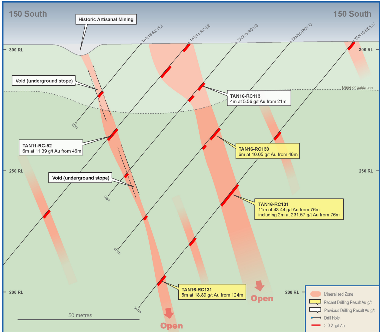
Figure 2: M1 Cross section – SE0150
