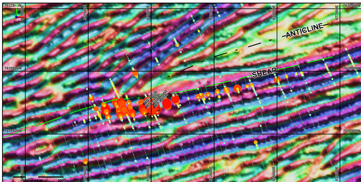
Figure 2: Magnetic image of Tshimologo (T4) showing 2-3km long Cu Soil Anomaly, interpreted regional shear zone and location of MOD/MTR drill holes. (Note: UTM grid lines are spaced 2.5km apart in image)
