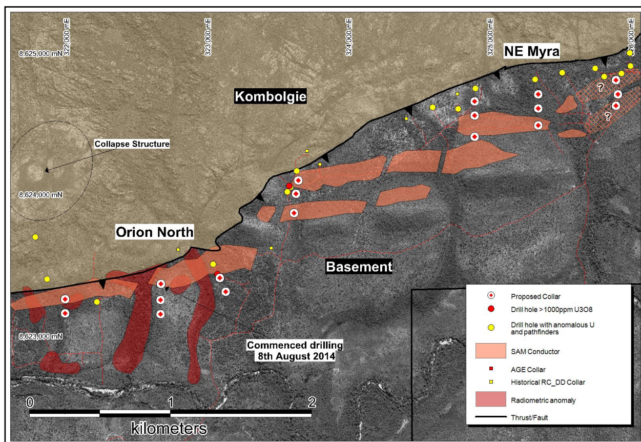
Figure 1. Orion North / NE Myra Target areas and Planned Drilling Locations
