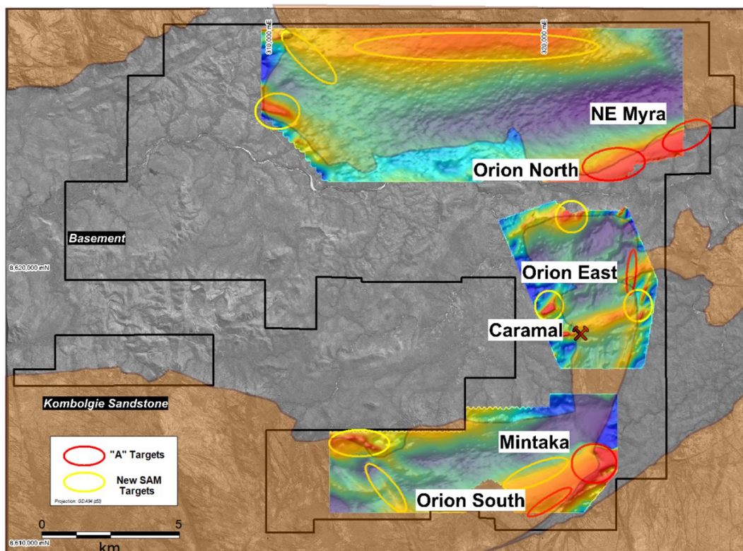
Figure 2. Tin Camp Creek Project area and Image of MMR responses. Red and orange coloured areas relate to low resistivity/higher conductivity.
