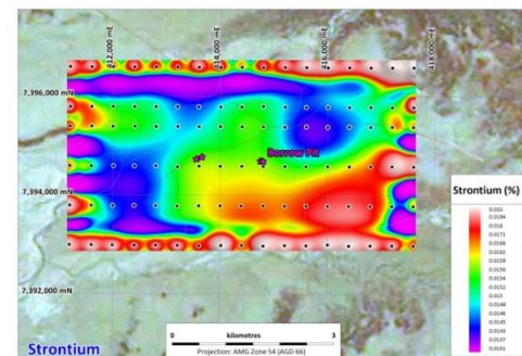
n.b. pink starts are anomalous rare earth recon samples Coorabulka EPM19286 - Soil Sampling XRF Results FIGURE 2
