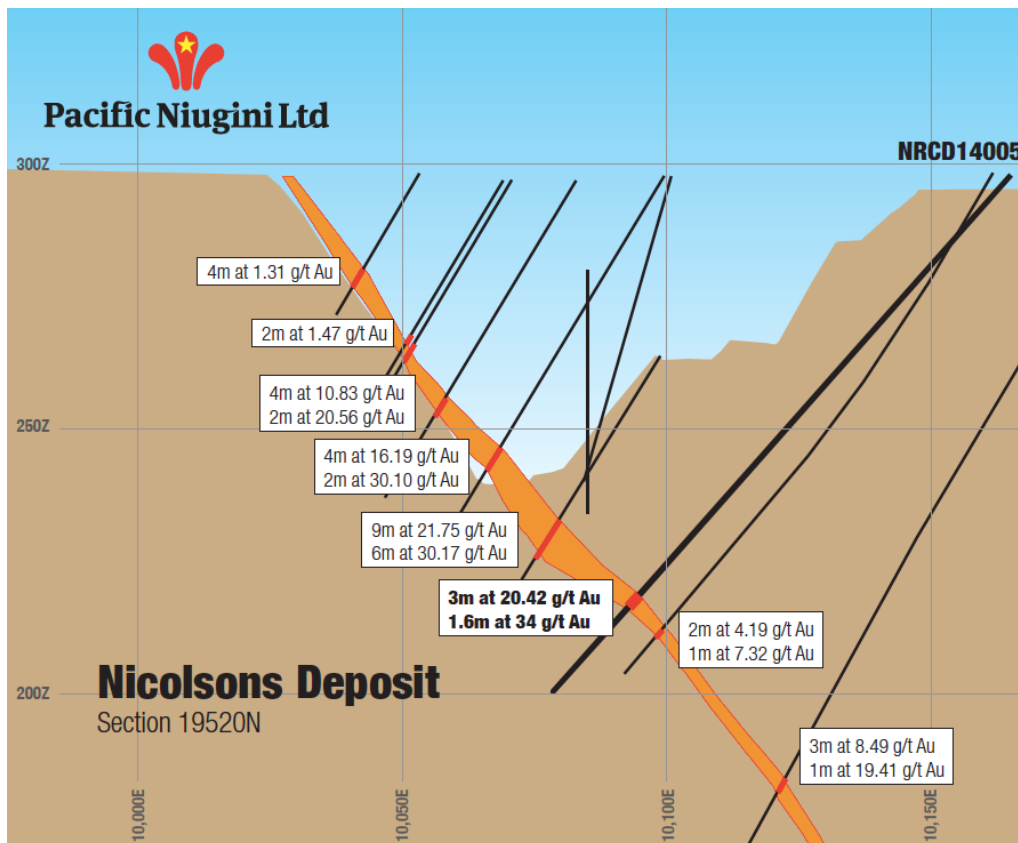
Interpreted ore section at 19520N showing historical RC results and current diamond drilling result from NRCD14005
