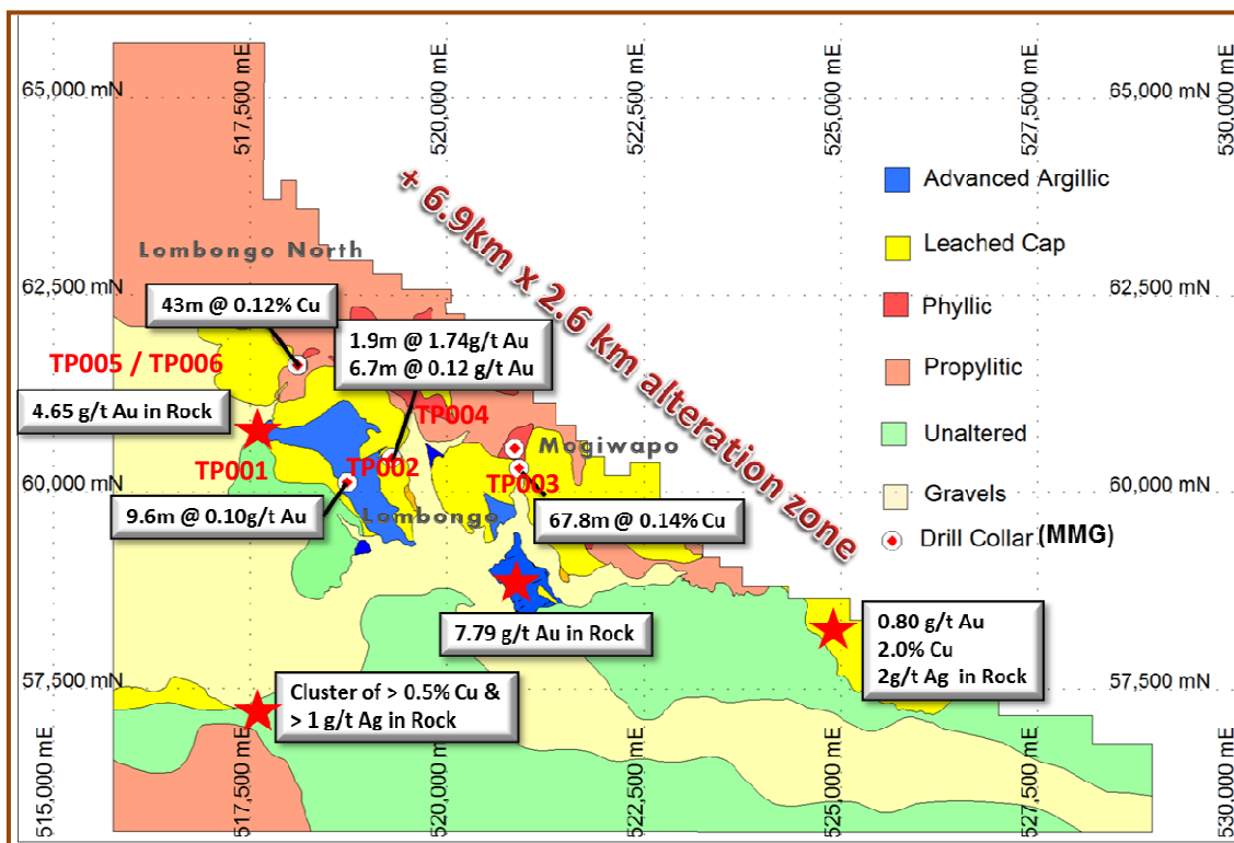
Tapadaa property map from MMG showing mapped alteration zones and MMG drill hole locations with significant intercepts.
