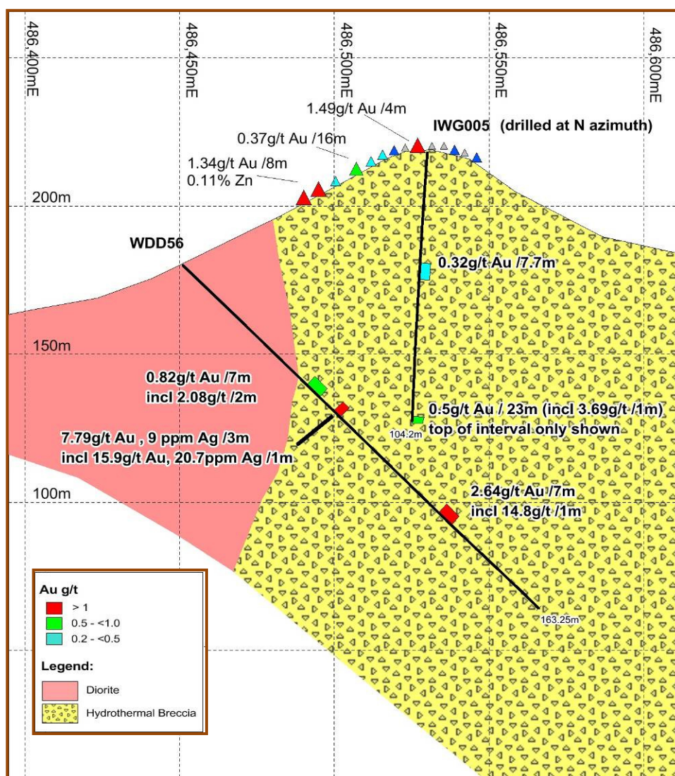
Interpreted geological cross section of WDD056 looking north. Note that only partial Oxindo (IWG005) hole trace is shown in the section as it was drilled at north azimuth. Section window is 50 metres in width. Trench chip samples intervals are also shown.
