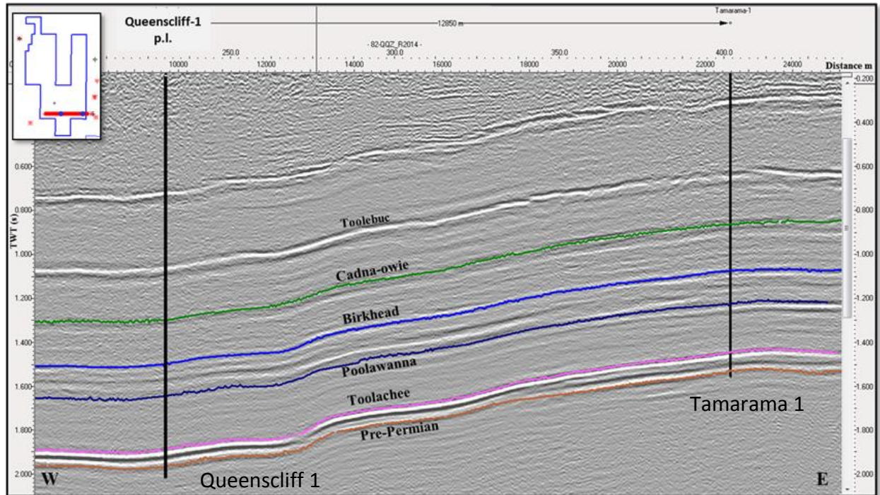
Figure 3 – Seismic Section with Proposed Tamarama-1 and Queenscliff-1 Locations
