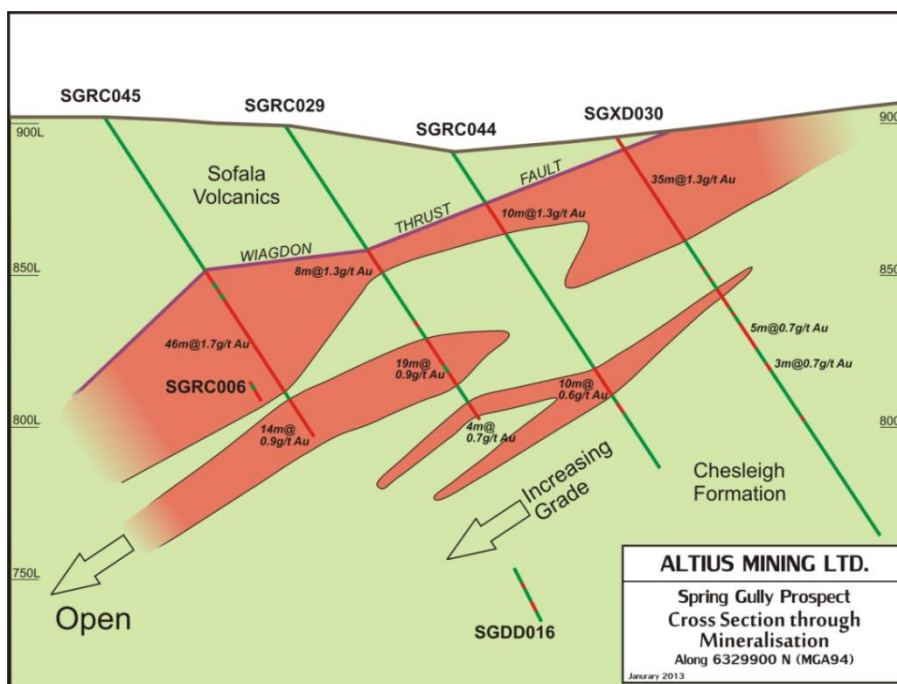
Figure 5: Cross section, with RGC drillholes, through the Spring Gully mineralisation (6329900 North) Note: AUML has no knowledge of the quality of the data used to produce this cross section.
