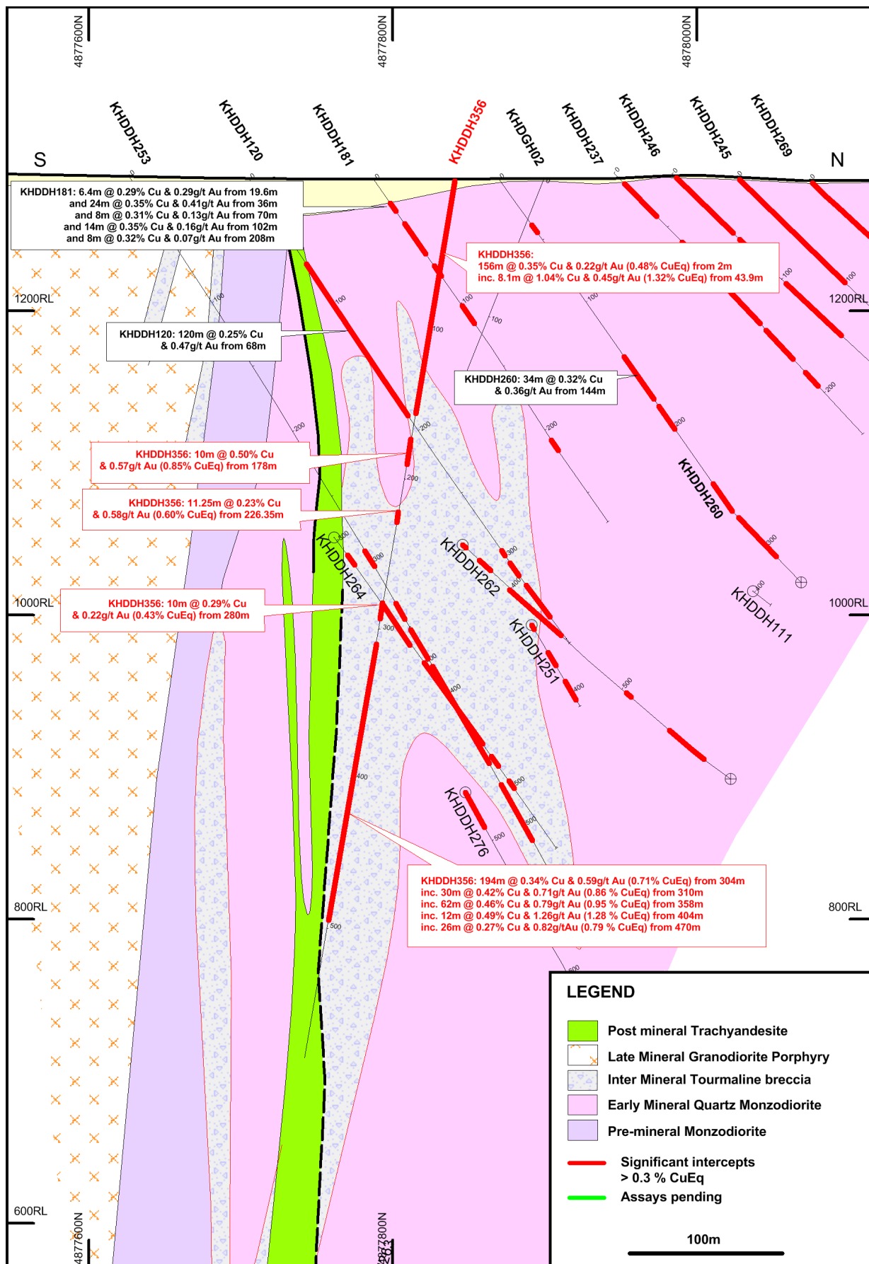
FIGURE 3: CROSS SECTIONSHOWING MINERALISATION AT SURFACE
