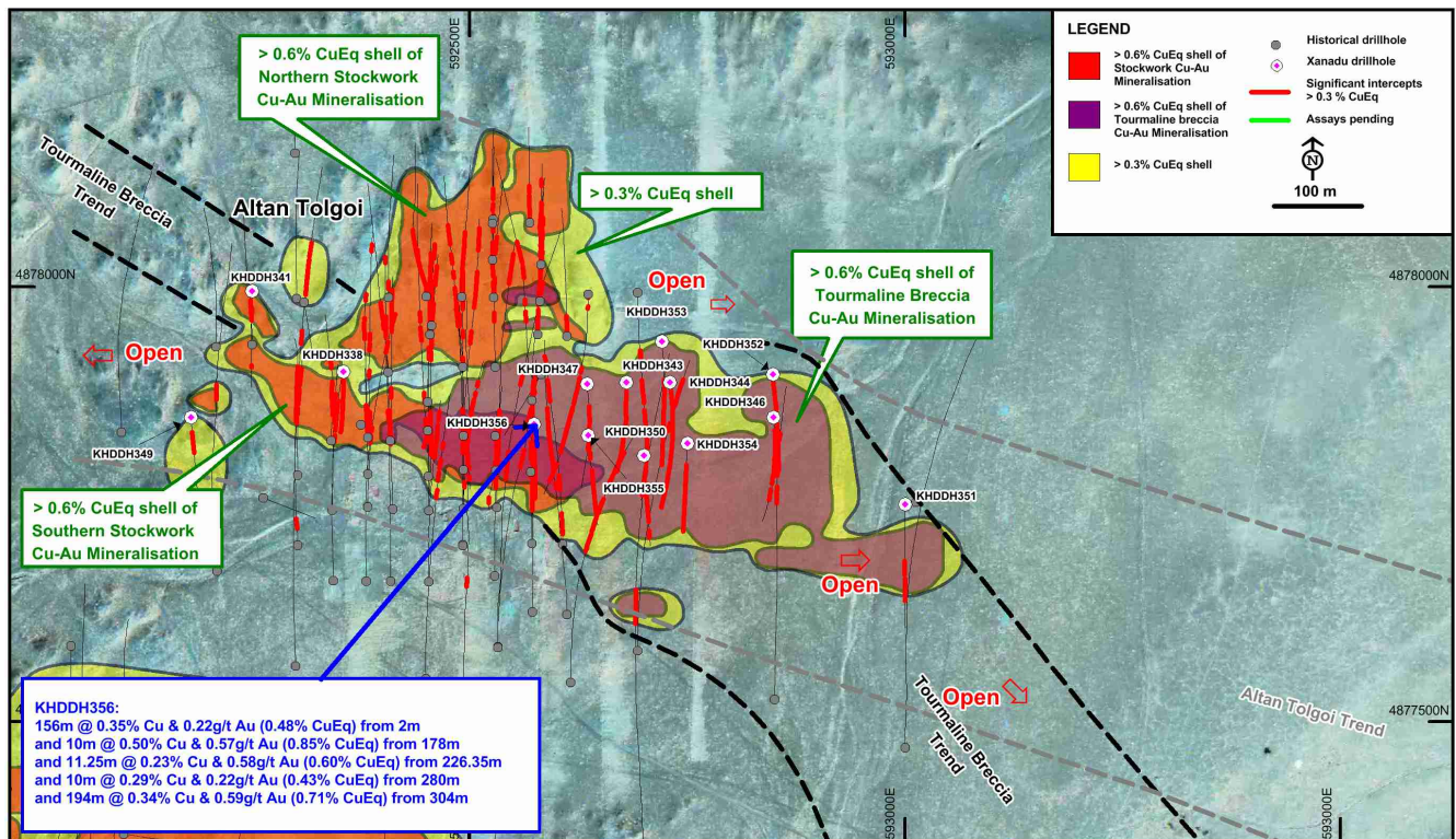
FIGURE1: ALTAN TOLGOI PLAN
