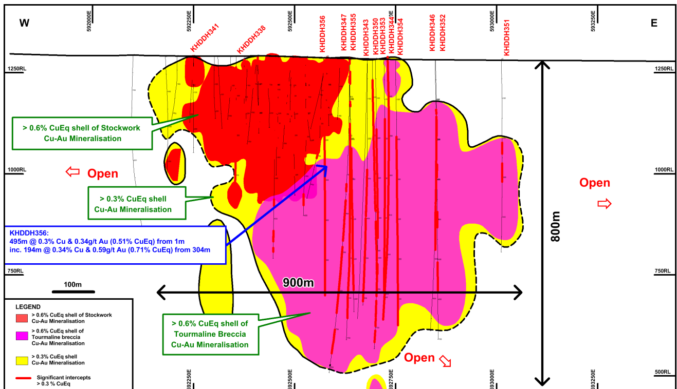
FIGURE2: ALTAN TOLGOI LONG SECTION
