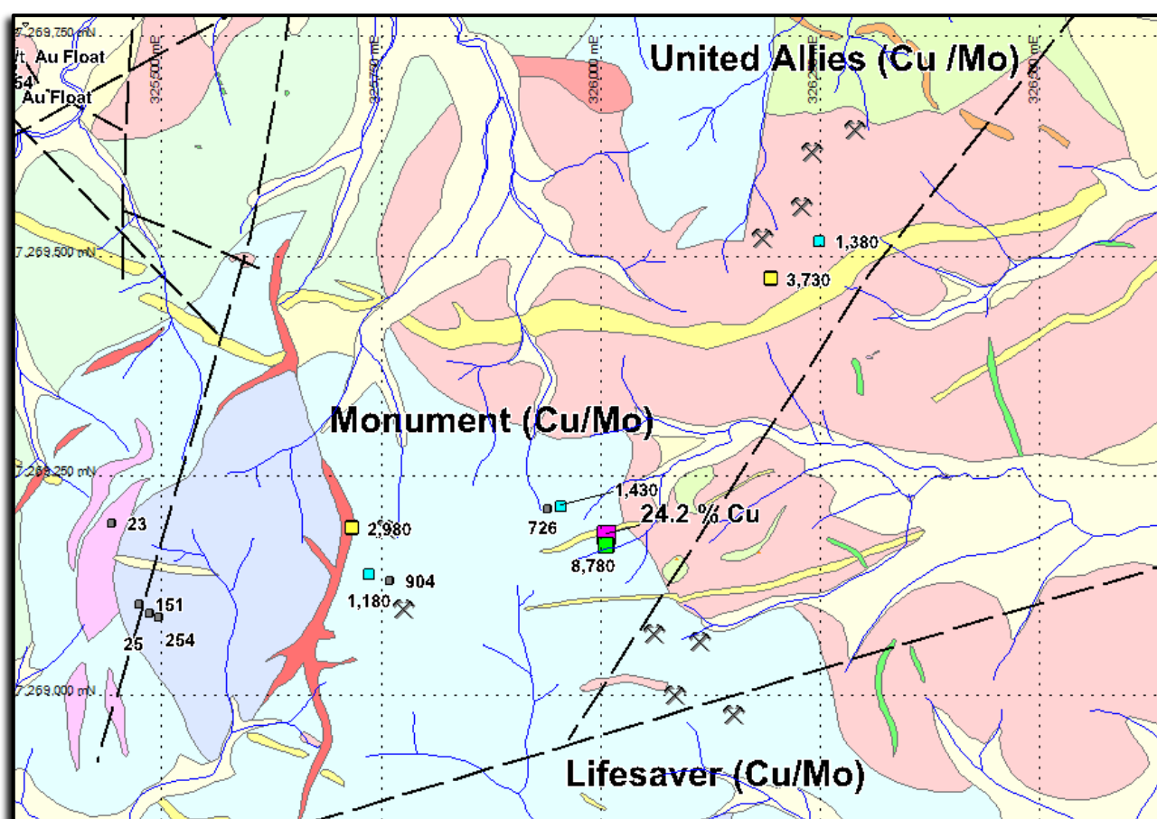
Figure 2. Location of recent rock chip samples with copper results displayed (ppm). Monument Intrusive Body in pink.
