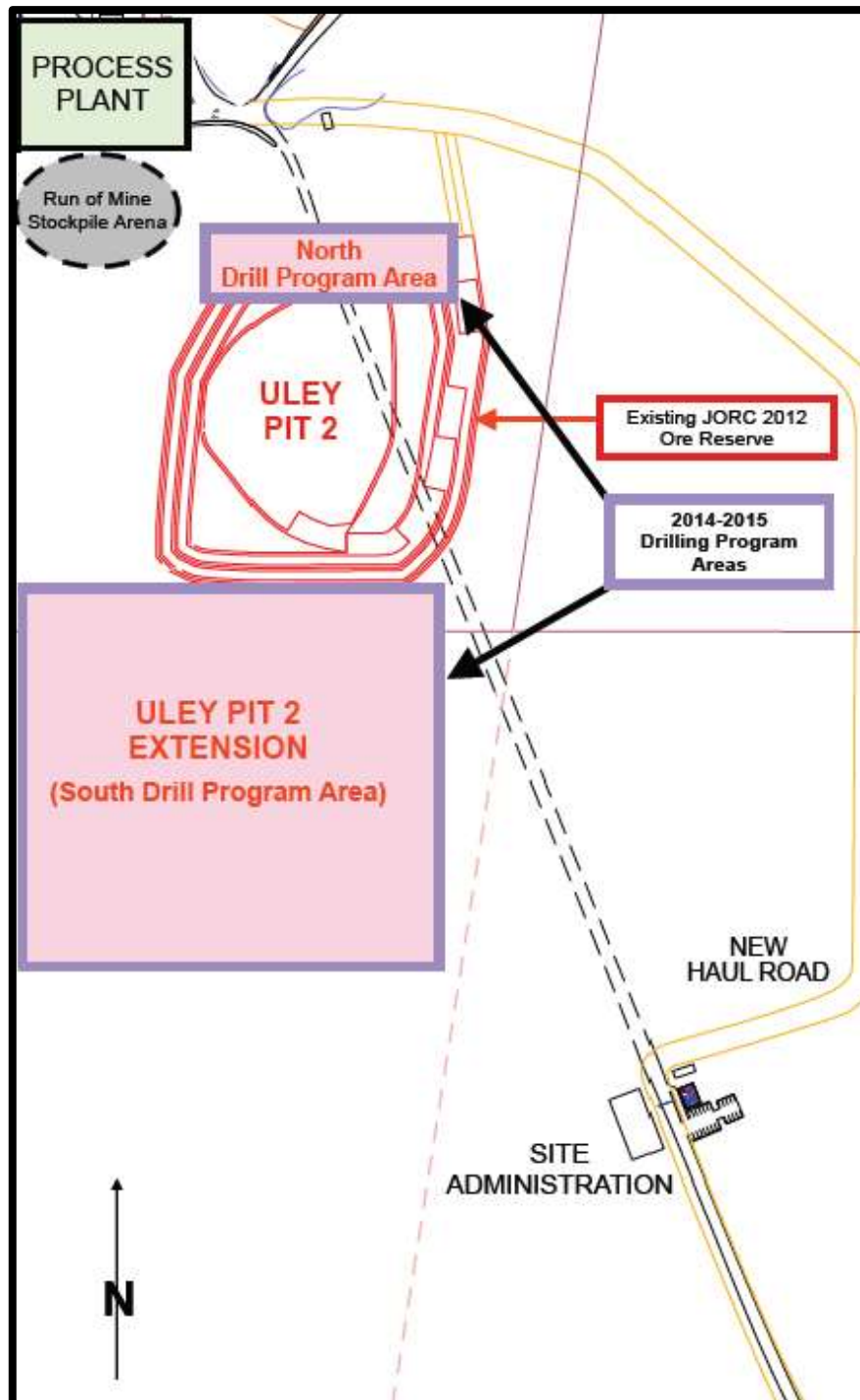
Figure 1 – Indicative site context of assays reported (not to scale).
