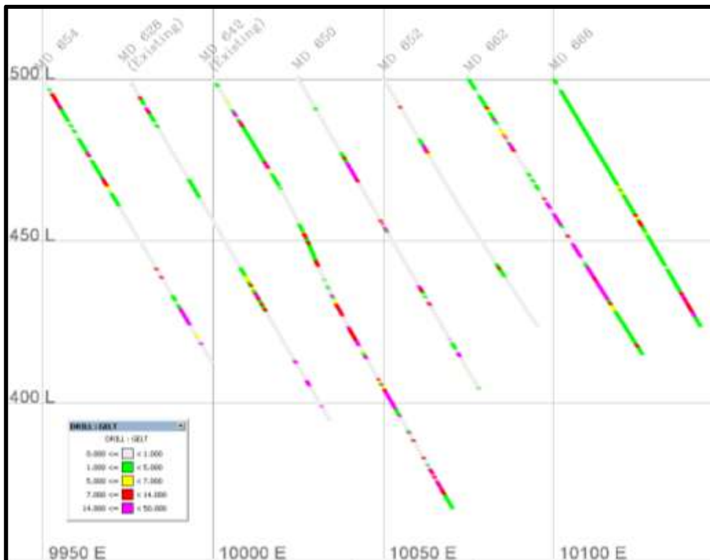
Figure 7: Assay Section 9550N (legend in % graphitic Carbon)
