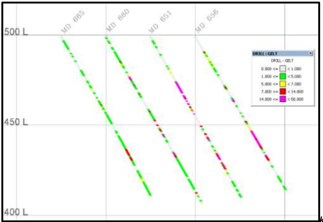
Figure 8: Assay Section 9350N (legend in % graphitic Carbon)
