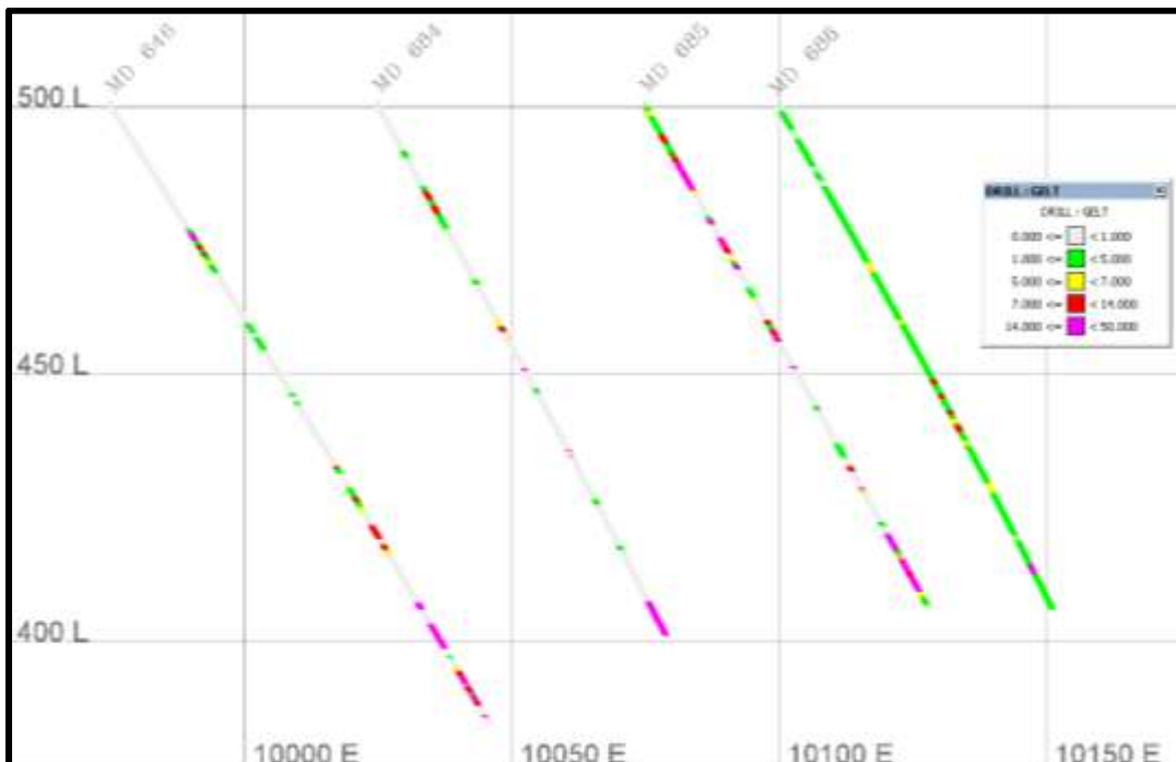
Figure 5: Assay Section 9600N (legend in % graphitic Carbon)
