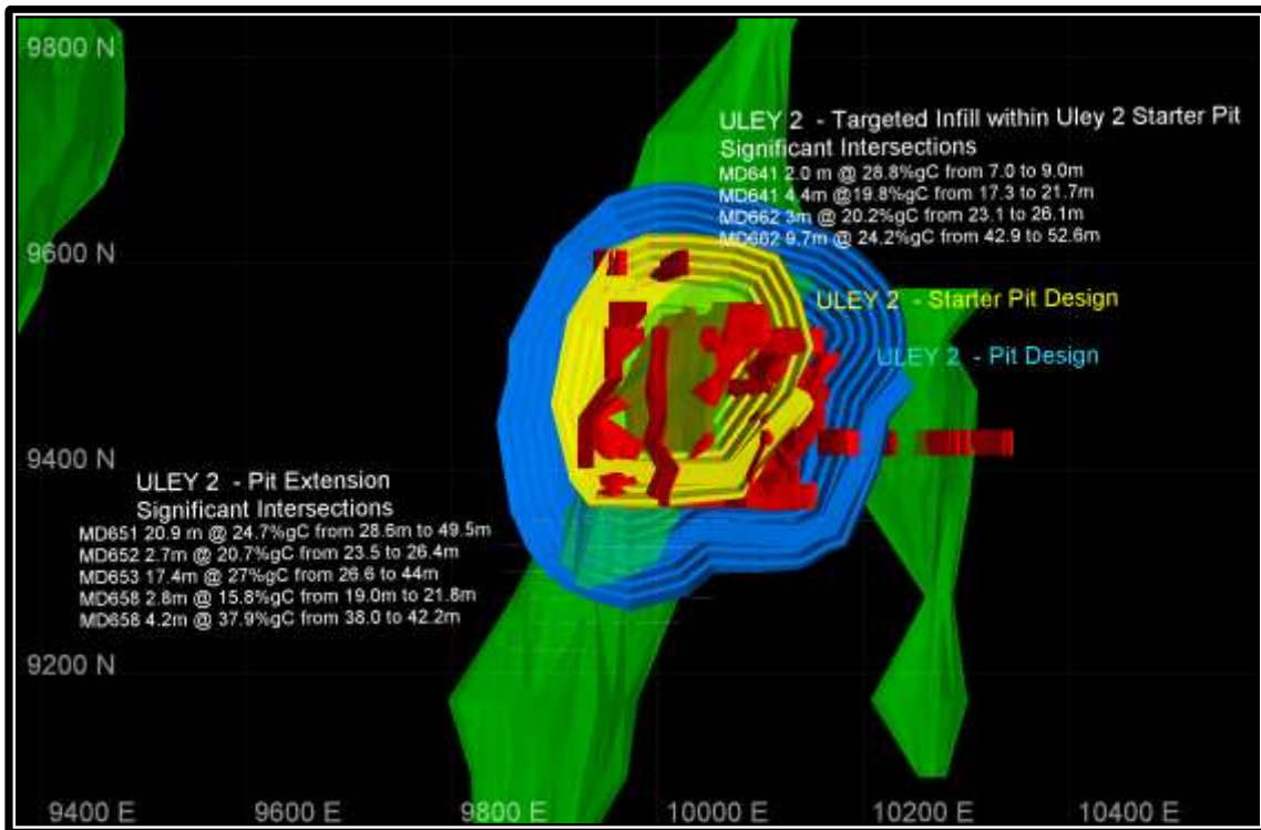
Figure 2 – Geological and Mining context of assays reported.
