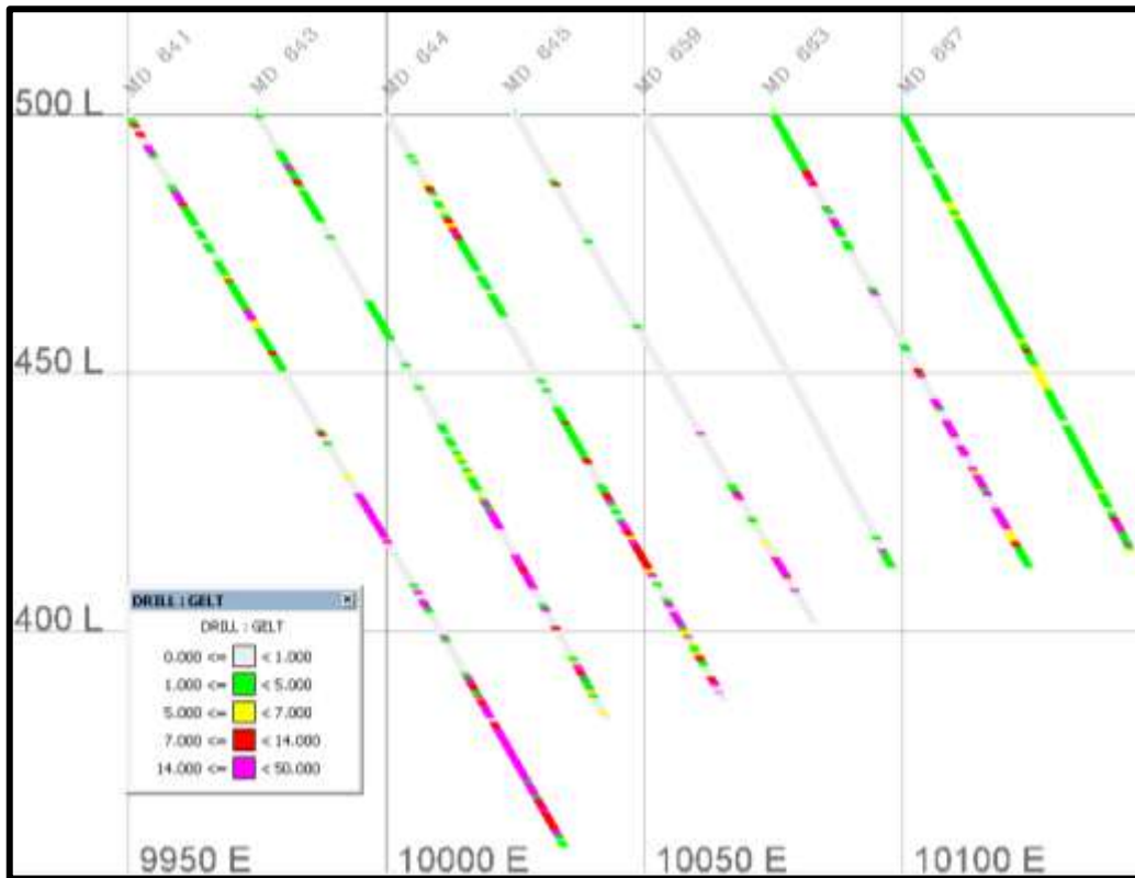
Figure 6: Assay Section 9575N (legend in % graphitic Carbon)
