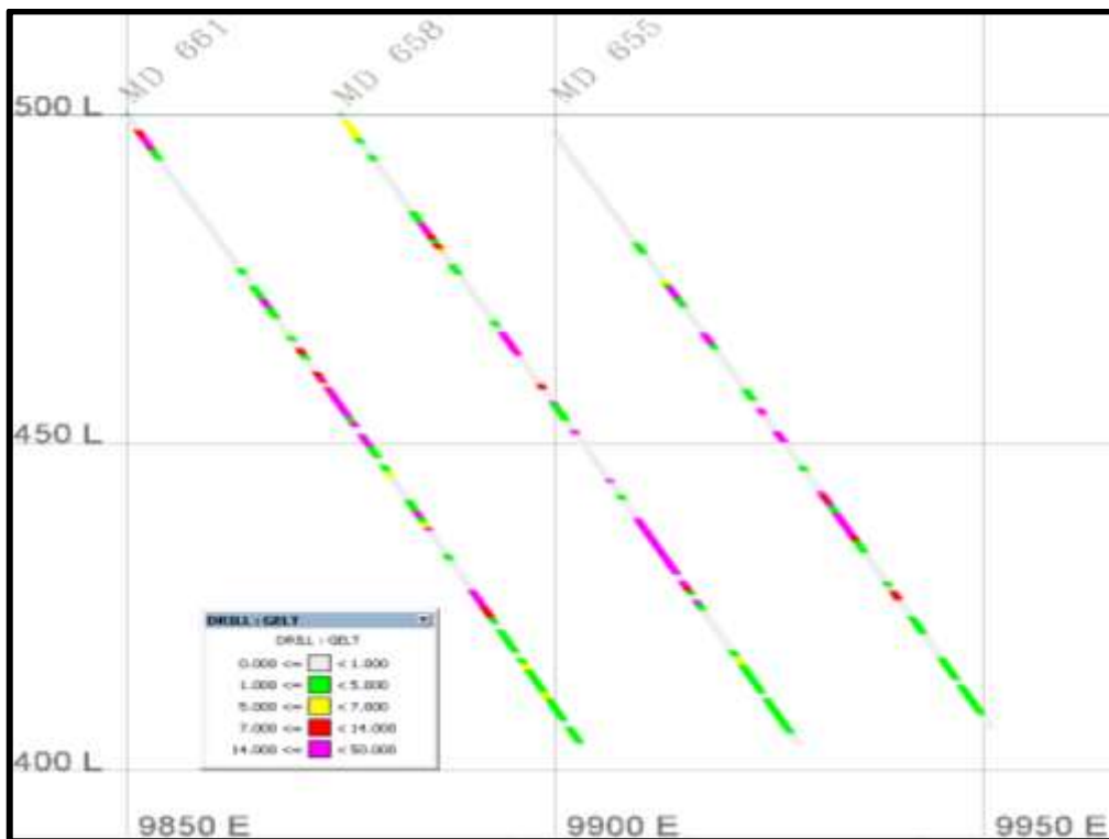
Figure 9: Assay Section 9225N (legend in % graphitic Carbon)
