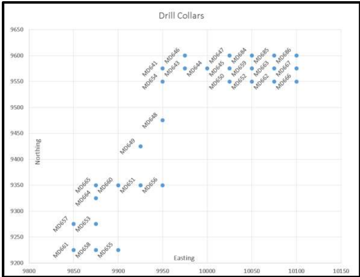
Figure 4 – Diamond Drill collar locations
