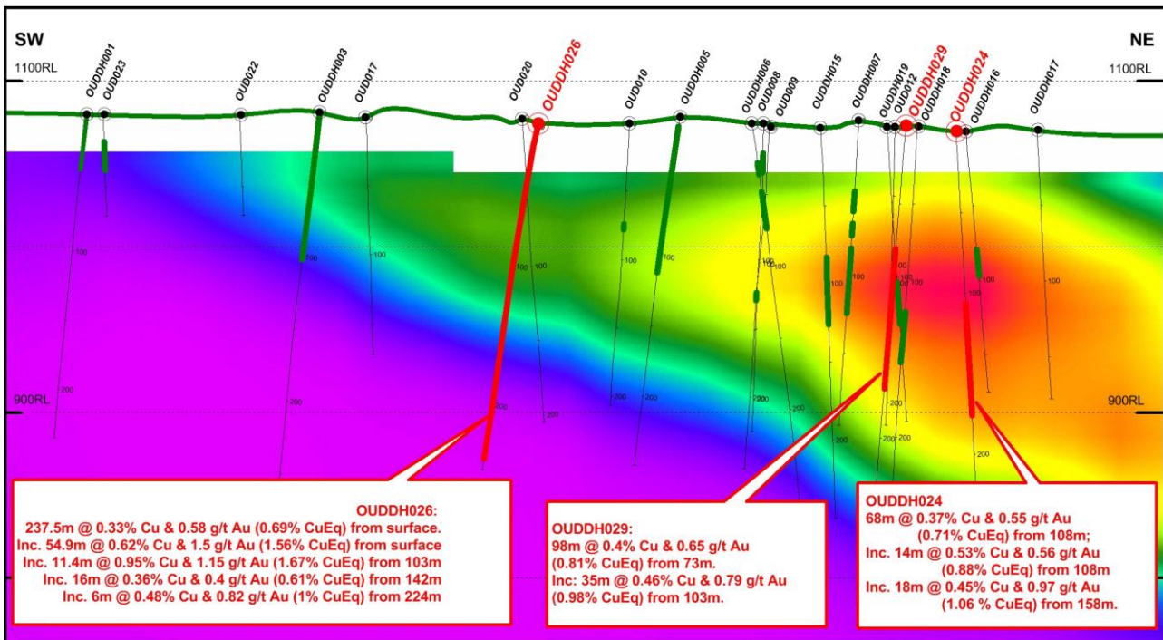
FIGURE 3: DIORITE HILL LONG SECTION SHOWING RECENT DRILL HOLES.
