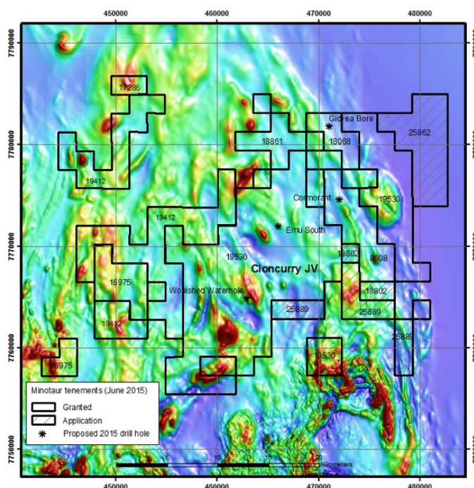
Figure 1: Emu South, Gidyea Bore, Cormorant and Woolshed Waterhole drill targets over aeromagnetic image.
