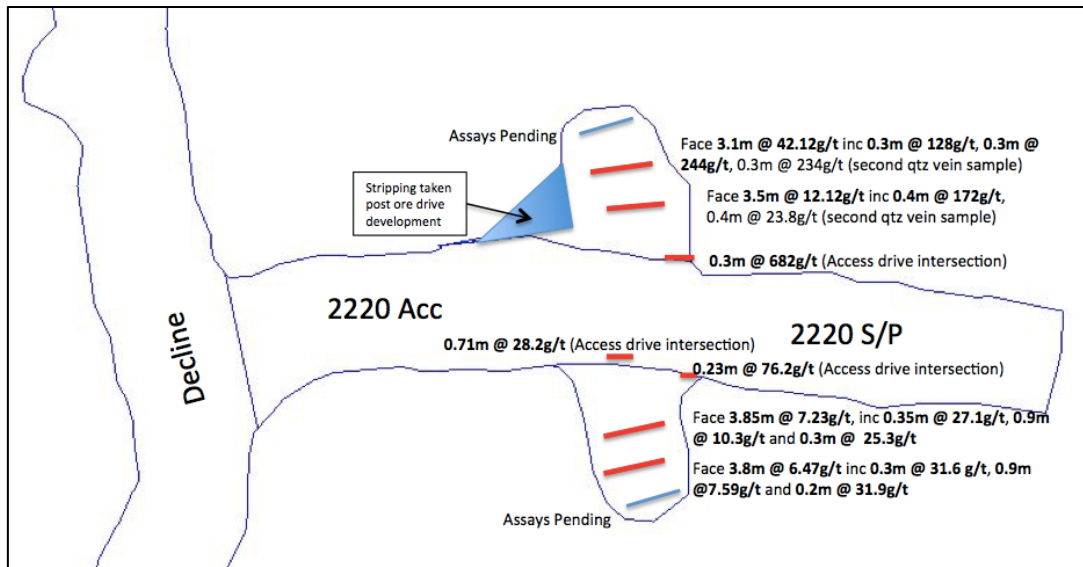
2220 Level Development as at 20/7/2015
