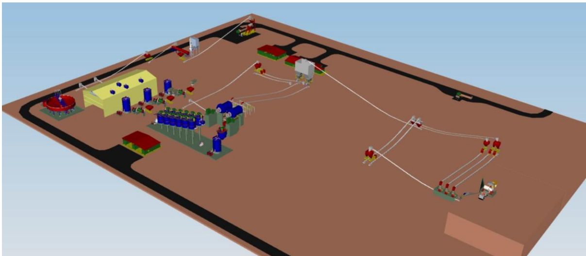
Figure 7 – Draft 3D Mechanical Layout of 250,000 tpa graphite concentrate plant
