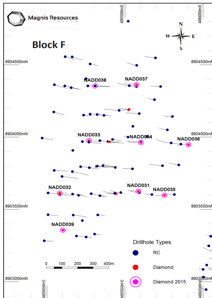
Figure 6 – Recently completed resource diamond core drill holes in Block F
