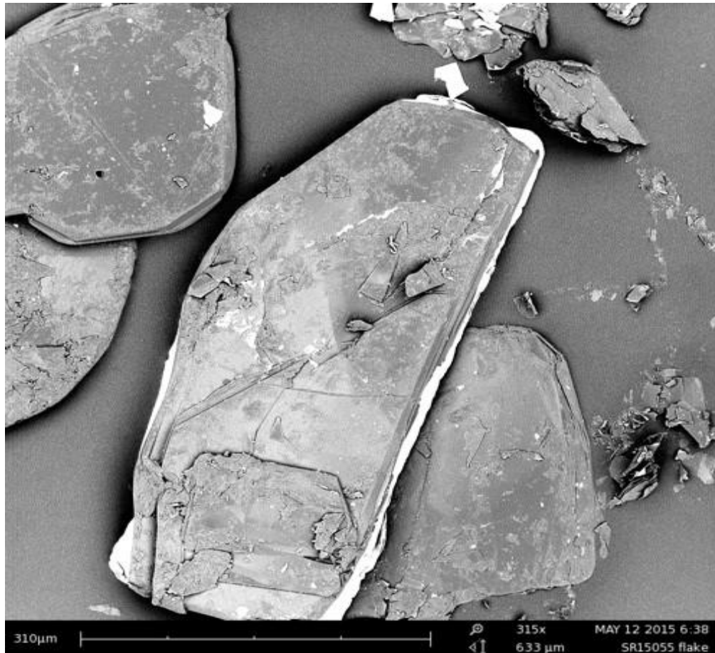
Figure 8 – Super Jumbo Flake size (defined as >500 microns) from the Nachu Graphite Project observed under a magnified microscope x 315 power. Of note is the uniformity of the graphite crystals with impurities at the surface which simplifies downstream purification.
