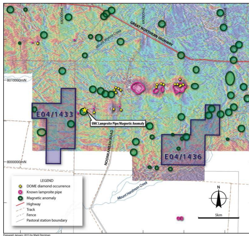
Figure 6: Known diamondiferous pipes and magnetic anomalies
