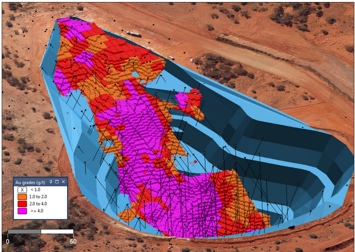
Figure 6: Mossbecker, 3D view to N, model, drilling & pit design
