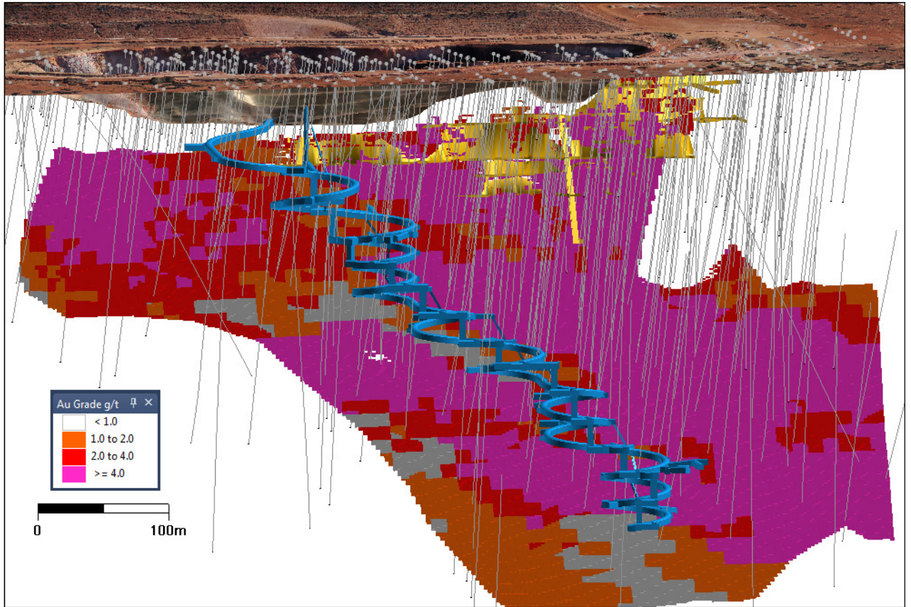
Figure 5: Vivien UG, 3D view to NW, model, drilling & decline
