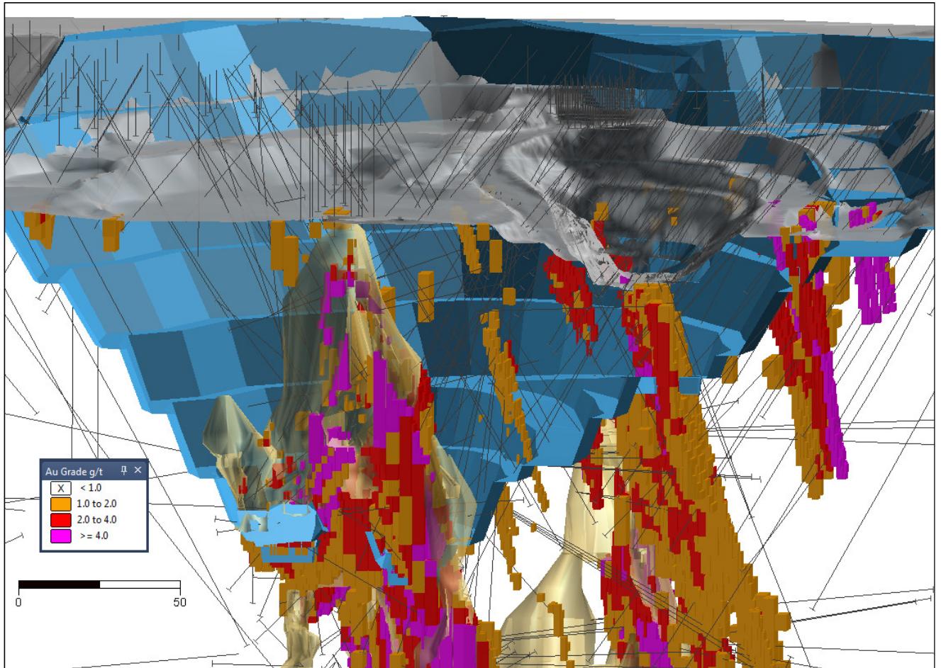
Figure 3: Perseverance (Galaxy), truncated view looking N, model, voids, drilling, pit design & June 2015 pit
