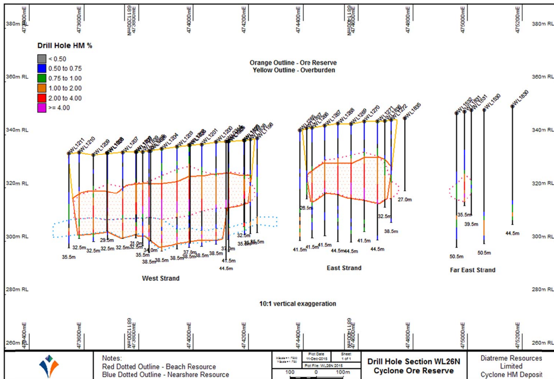
Figure 4: Drill Hole Section WL26N – Cyclone Ore Reserve
